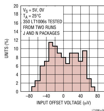
Distribution of Input Offset Voltage
