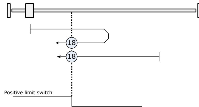
Figure 17: Homing Method 18
