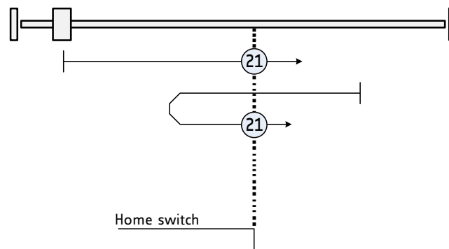
Figure 19: Homing Method 21
