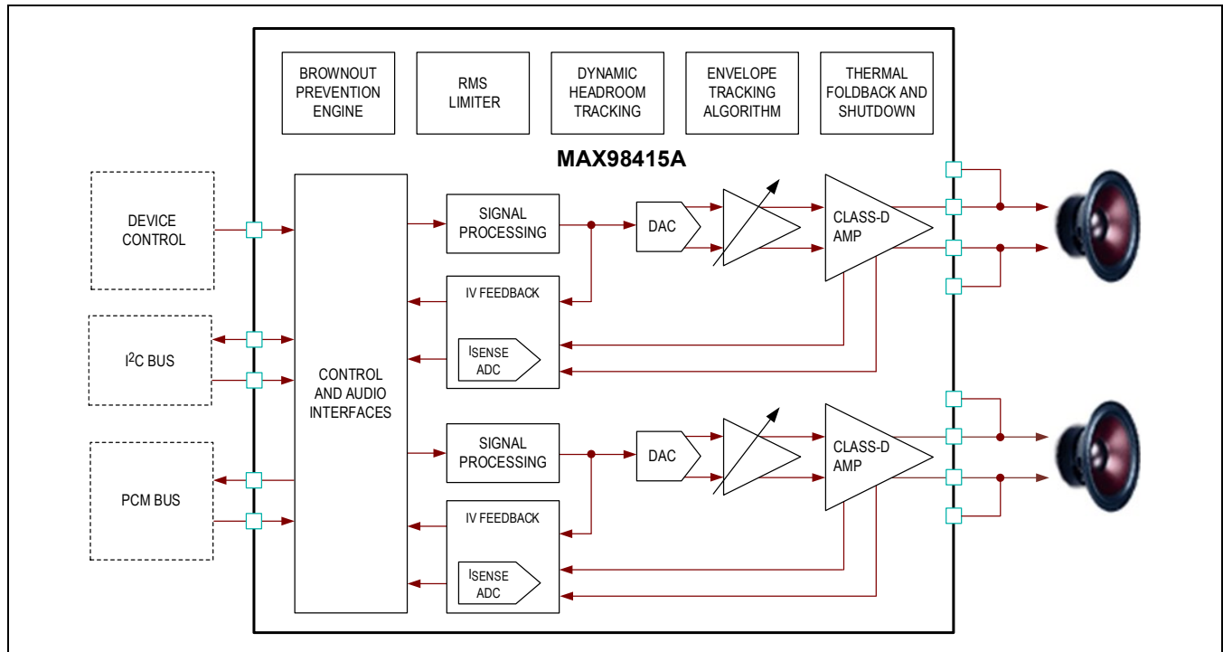
Figure 1. MAX98415A Simplified Block Diagram
