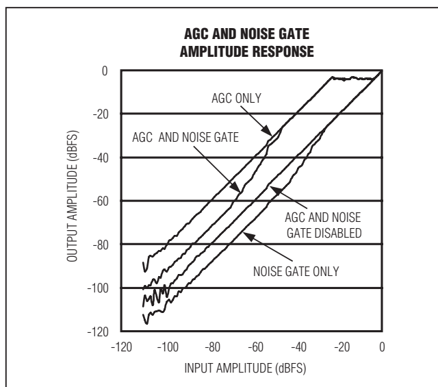
Figure 11. AGC and Noise Gate Input vs. Output Gain
