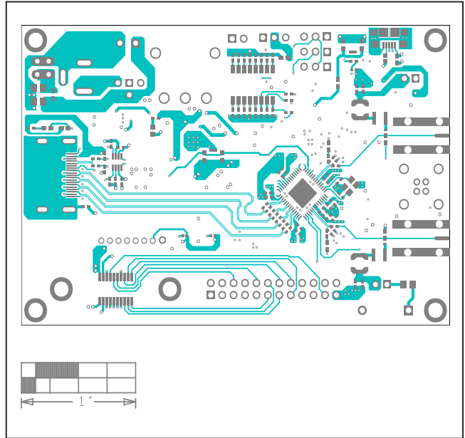
MAX96751 EV Kit PCB Layout—Top Layer
