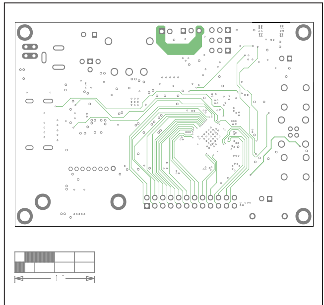
MAX96751 EV Kit PCB Layout—Internal 3
