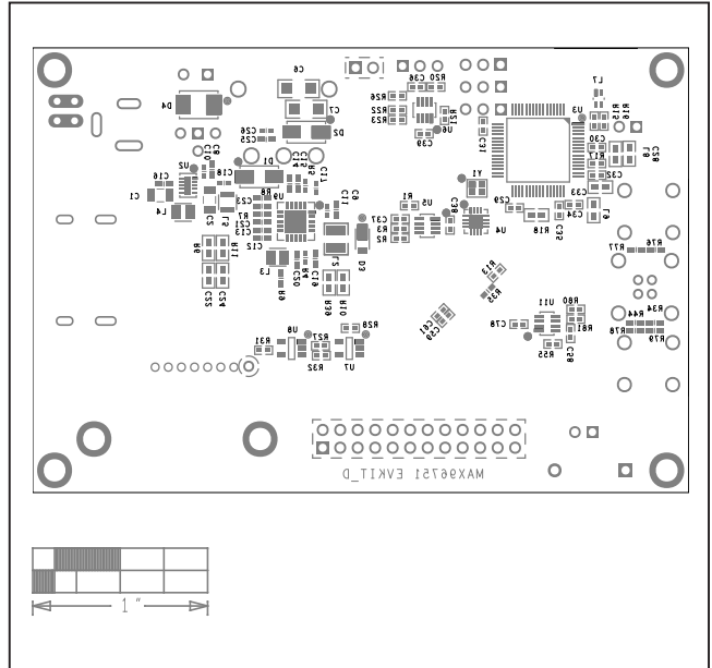
MAX96751 EV Kit PCB Layout—Bottom Silkscreen
