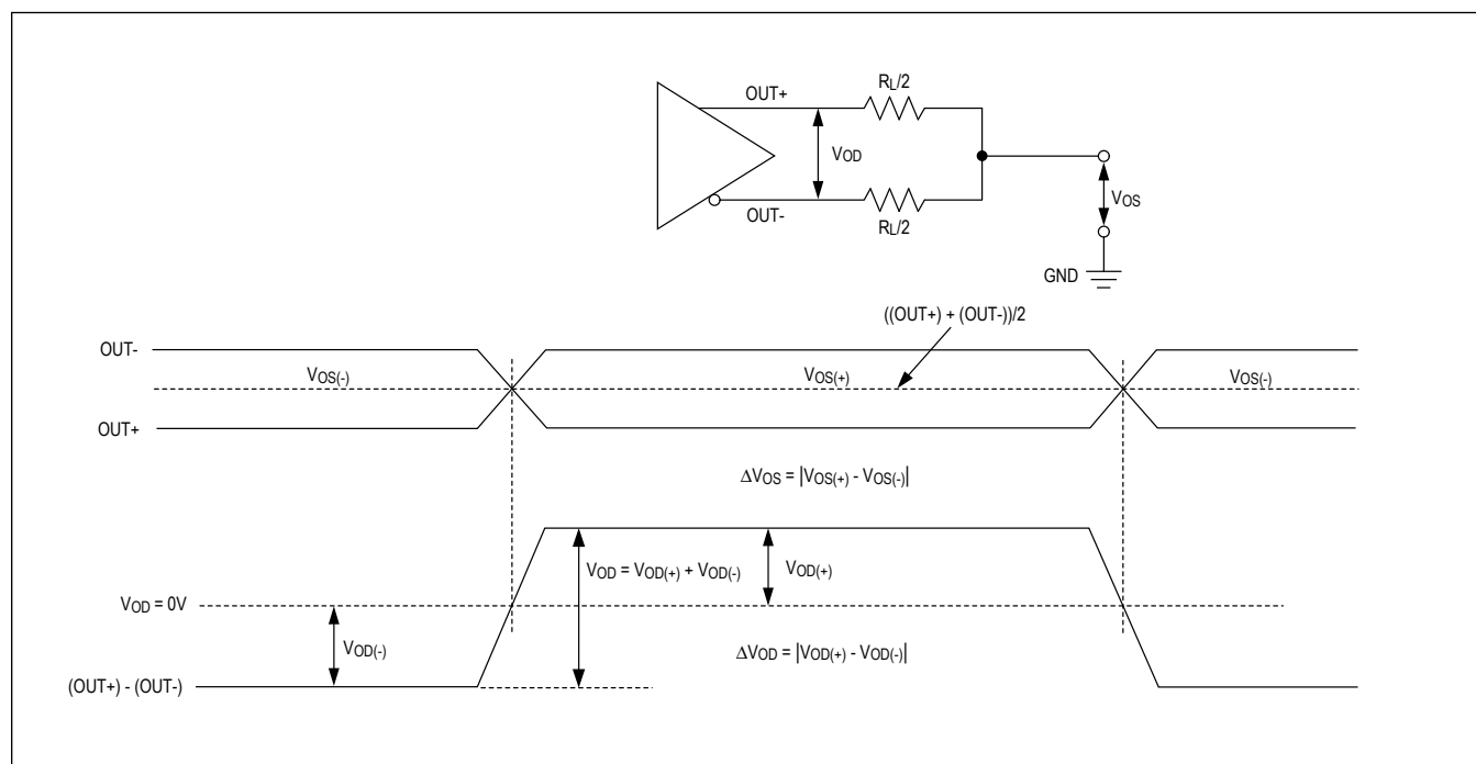
Figure 2. GMSL2 Reverse-Channel Serial Outputs
