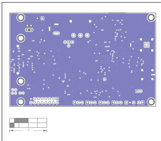
MAX9295D Coax/HSD EV Kit PCB Layout—L7 Ground
