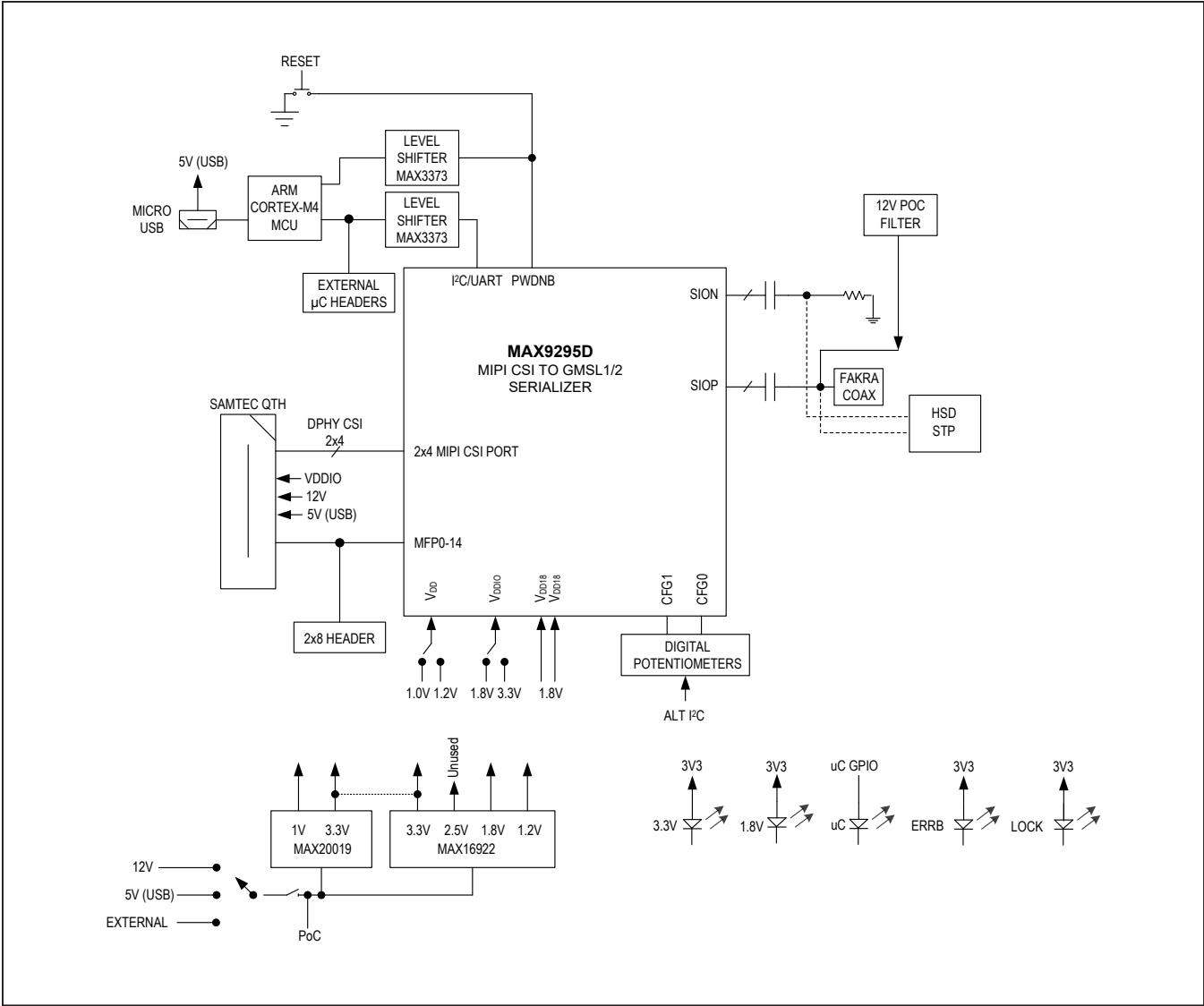
Figure 1. MAX9295D EV Kit Typical Block Diagram
