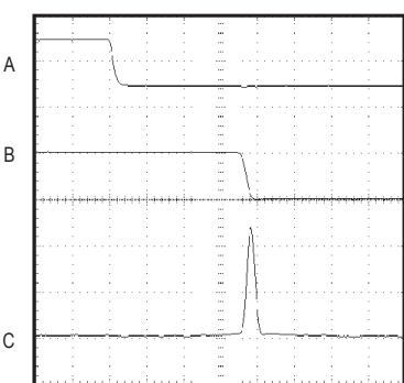
SWITCHING CURRENT (OUT FALLING EDGE)
