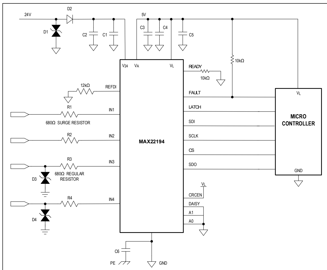
Figure 21. Typical EMC Protection Circuitry for the MAX22194
