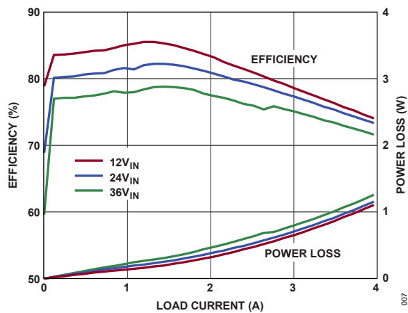
Figure 7. Efficiency vs. Power Loss, V_{OUT} = 0.8\text{V} , BIAS = 5V, Burst Mode Operation
