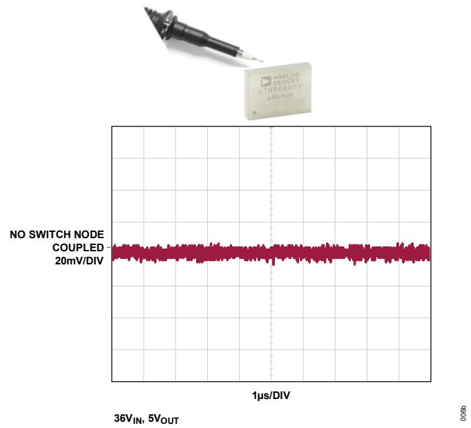
(b) LTM8060F with EMI Shielding
