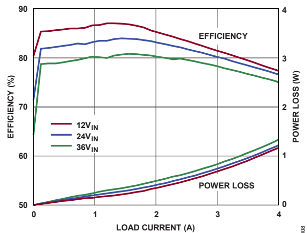
Figure 8. Efficiency vs. Power Loss, V_{OUT} = 1\text{V} , BIAS = 5V, Burst Mode Operation
