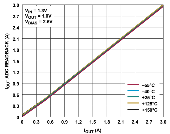
Figure 79. I_{OUT} ADC Readback
