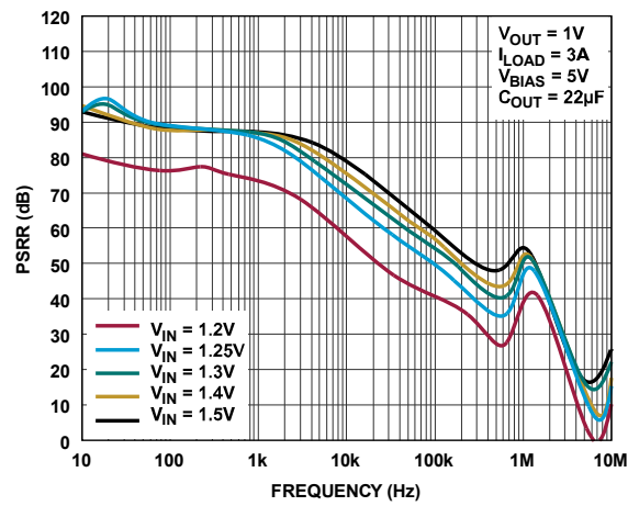
Figure 53. IN Pin PSRR
