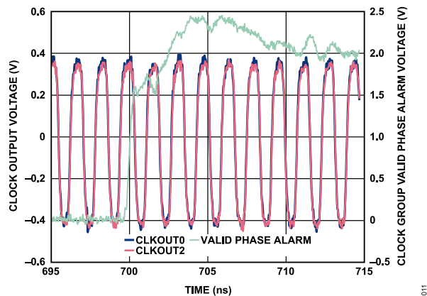
Figure 12. Output Channel Synchronization After Rephase
