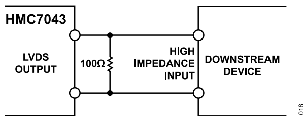
Figure 20. DC-Coupled LVDS Output Driver
