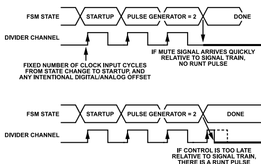
Figure 29. Start-Up Behavior of an Example Divider Configured as a Pulse Generator
