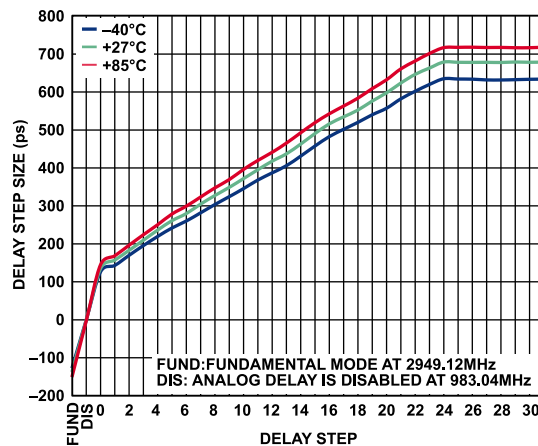
Figure 14. Analog Delay vs. Delay Setting over Temperature, LVPECL at 983.04 MHz
