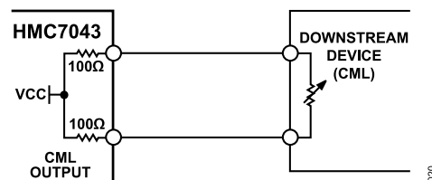
Figure 22. DC-Coupled CML (Internal) Output Driver
