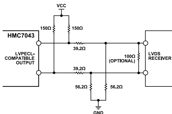
Figure 24. Level Translation for LVDS N-Pulse Operation (Place 100 Ω Termination Resistor If Receiver Does Not Have It.)
