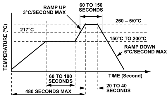
Figure 34. Pb-Free Reflow Solder Profile
