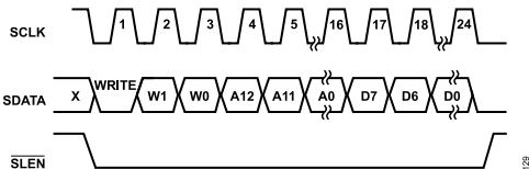
Figure 33. SPI Timing Diagram, Write Operation
