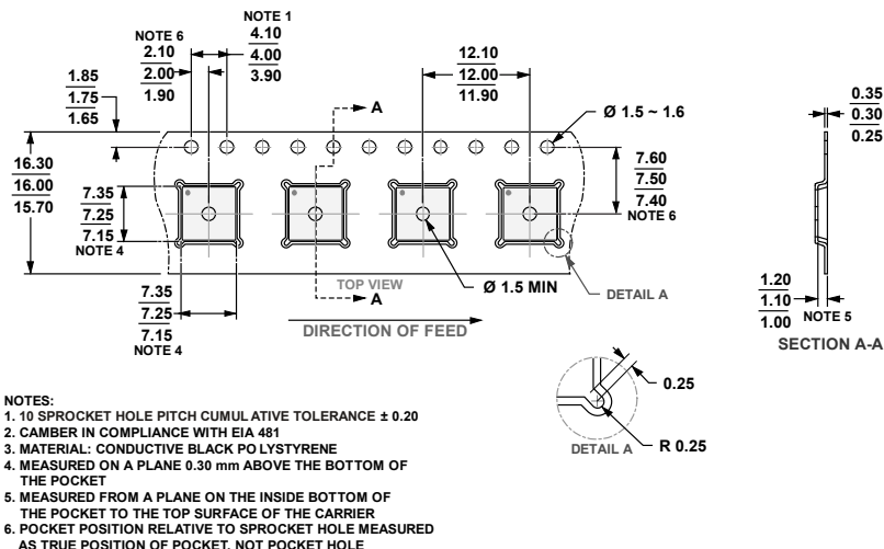
Figure 37. LFCSP Tape and Reel Outline Dimensions Dimensions shown in millimeters
