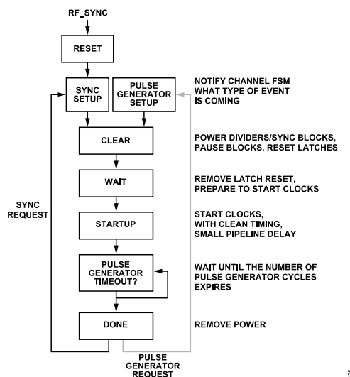
Figure 28. Synchronization FSM Flowchart
