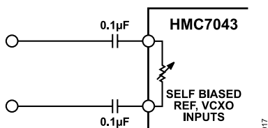
Figure 19. CLKIN/CLKIN, RFSYNCIN Input Differential Mode
