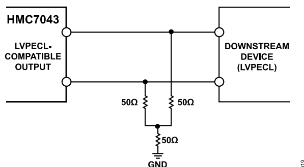
Figure 21. DC-Coupled LVPECL Output Driver
