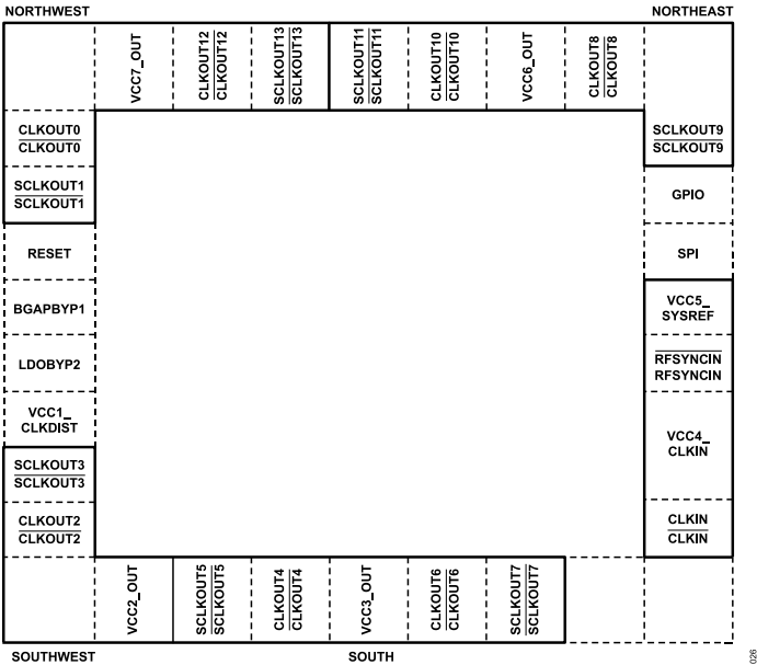
Figure 30. Clock Grouping
