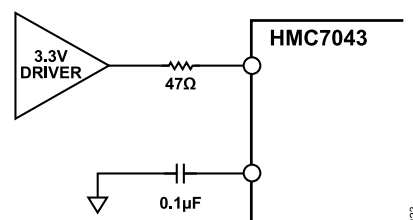
Figure 23. CLKIN, RFSYNCIN Input Single-Ended Mode
