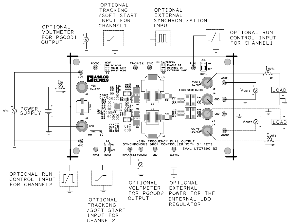
Figure 1. EVAL-LTC7890-BZ Board Connections
