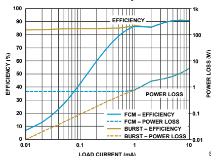
Figure 3. Channel 1 Efficiency vs. Load Current
