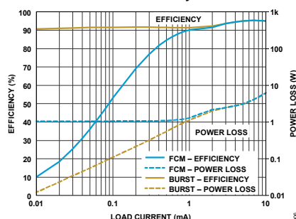
Figure 4. Channel 2 Efficiency vs. Load Current
