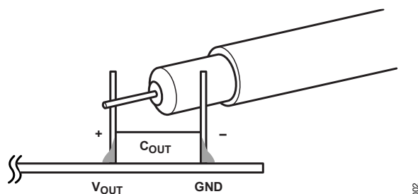
Figure 2. EVAL-LTC7890-BZ Ripple Measurement
