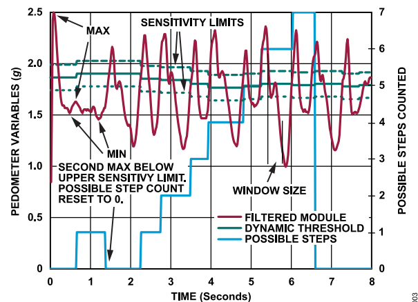
Figure 46. Step Counter Acceleration Signal Processing
