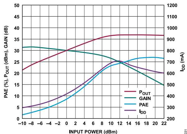
Figure 31. PAE, P_{OUT} , Gain, and Supply Current ( I_{DD} ) vs. Input Power at 0.3 GHz, V_{DD} = 28 \text{ V} , I_{DQ} = 300 \text{ mA}
