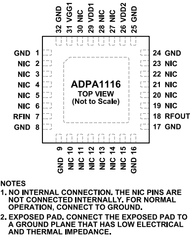
Figure 2. Pin Configuration
