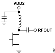
Figure 6. VDD2 and RFOUT Interface Schematic
