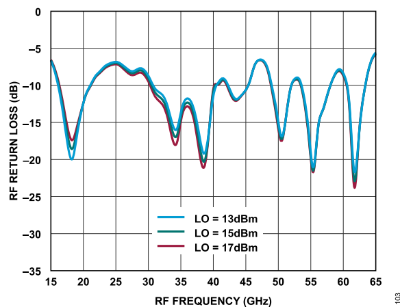
Figure 103. RF Return Loss vs. RF Frequency at Various LO Power Levels, T_A = 25^\circ\text{C} , LO = 40 GHz
