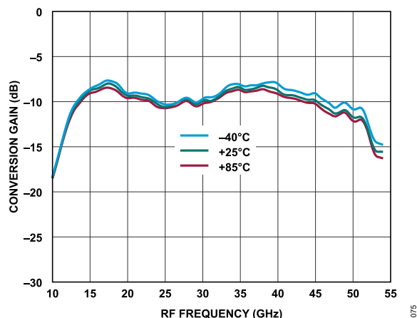
Figure 75. Conversion Gain vs. RF Frequency at Various Temperatures, LO = 15 dBm
