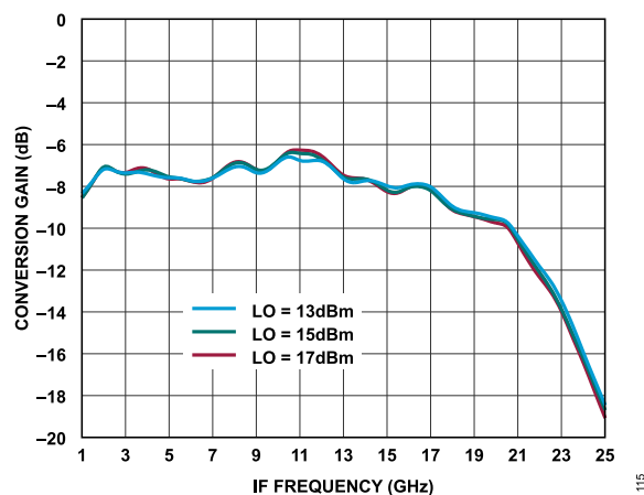
Figure 115. Conversion Gain vs. IF Frequency at Various LO Power Levels, T_A = 25^\circ\text{C}
