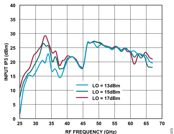
Figure 73. Input IP3 vs. RF Frequency at Various LO Power Levels, T_A = 25^\circ\text{C}
