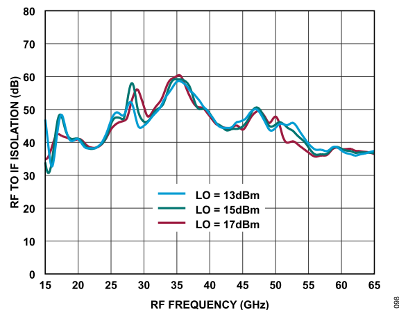
Figure 98. RF to IF Isolation vs. RF Frequency at Various LO Power Levels, T_A = 25^\circ\text{C}
