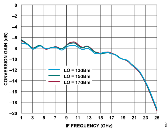
Figure 107. Conversion Gain vs. IF Frequency at Various LO Power Levels, T_A = 25^\circ\text{C}
