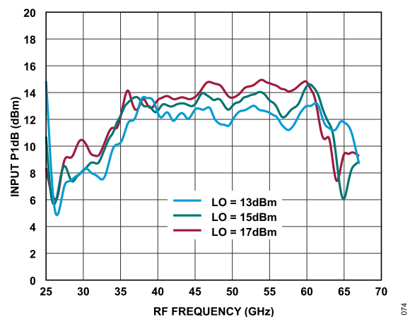
Figure 74. Input P1dB vs. RF Frequency at Various LO Power Levels, T_A = 25^\circ\text{C}
