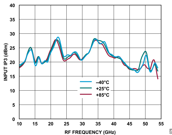
Figure 76. Input IP3 vs. RF Frequency at Various Temperatures, LO = 15 dBm
