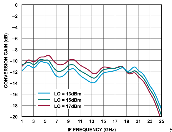
Figure 111. Conversion Gain vs. IF Frequency at Various LO Power Levels, T_A = 25^\circ\text{C}
