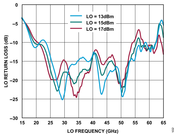
Figure 102. LO Return Loss vs. LO Frequency at Various LO Power Levels, T_A = 25^\circ\text{C}
