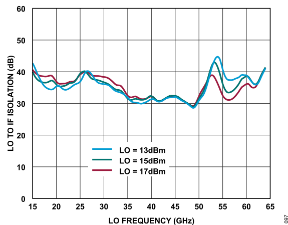
Figure 97. LO to IF Isolation vs. LO Frequency at Various LO Power Levels, T_A = 25^\circ\text{C}
