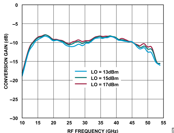
Figure 78. Conversion Gain vs. RF Frequency at Various LO Power Levels, T_A = 25^\circ\text{C}
