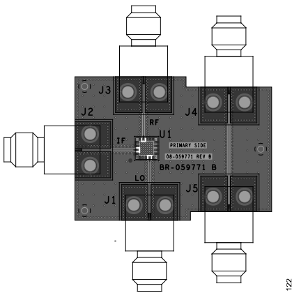
Figure 122. Evaluation PCB Top Layer
