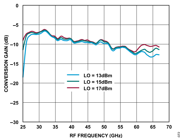
Figure 72. Conversion Gain vs. RF Frequency at Various LO Power Levels, T_A = 25^\circ\text{C}
