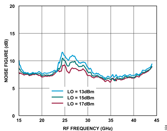
Figure 24. Noise Figure vs. RF Frequency at Various LO Power Levels, T_A = 25^\circ\text{C}
