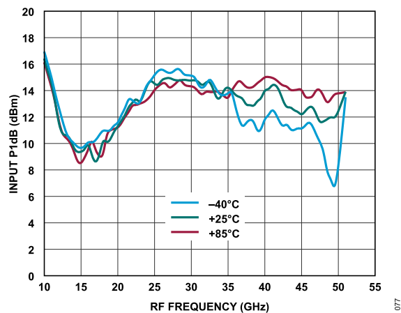
Figure 77. Input P1dB vs. RF Frequency at Various Temperatures, LO = 15 dBm
