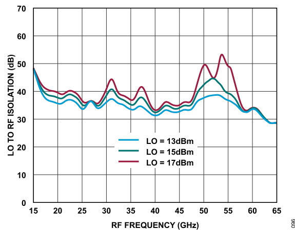
Figure 96. LO to RF Isolation vs. RF Frequency at Various LO Power Levels, T_A = 25^\circ\text{C}
