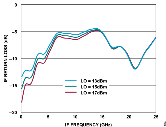
Figure 104. IF Return Loss vs. IF Frequency at Various LO Power Levels, T_A = 25^\circ\text{C} , LO = 40 GHz
