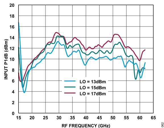
Figure 62. Input P1dB vs. RF Frequency at Various LO Power Levels, T_A = 25^\circ\text{C}
