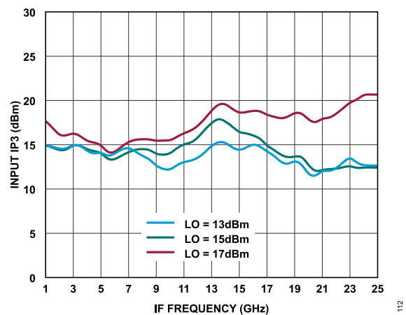
Figure 112. Input IP3 vs. IF Frequency at Various LO Power Levels, T_A = 25^\circ\text{C}
