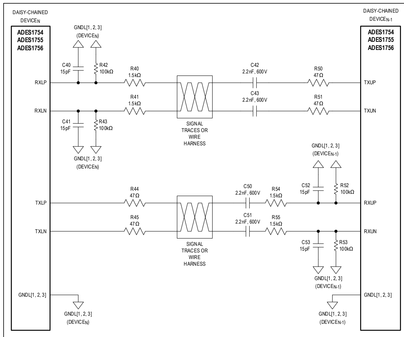
Figure 100. UART Connection
