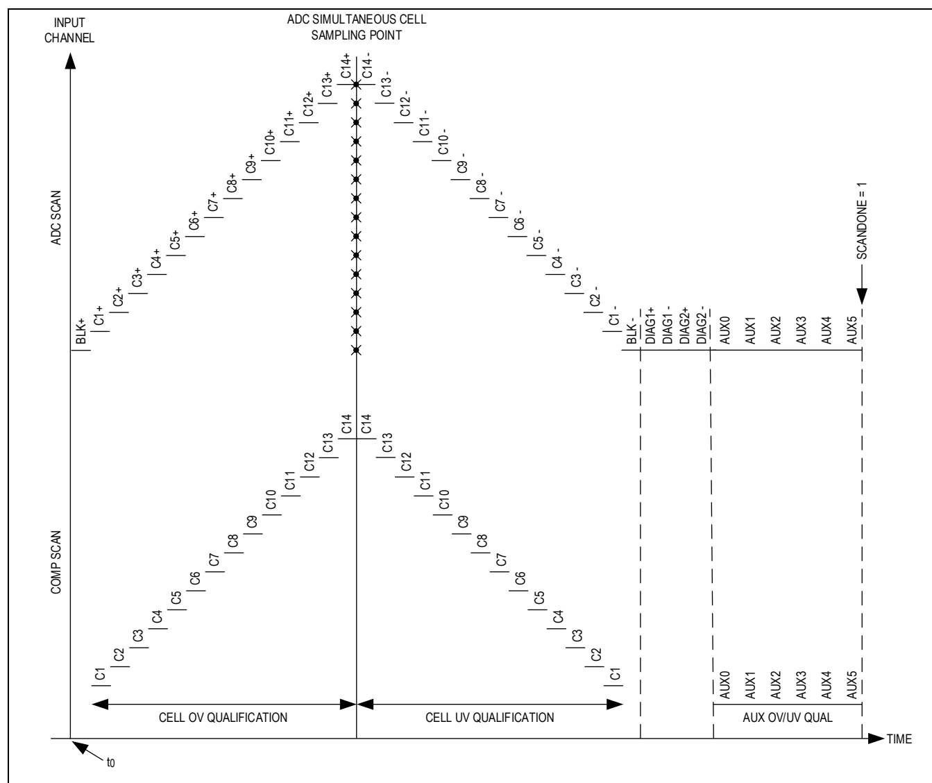
Figure 24. Simultaneous ADC+COMP Scan Mode
