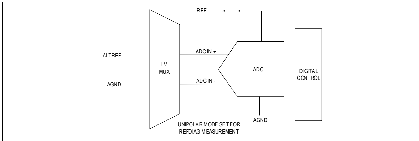
Figure 74. ALTREF Diagnostic
