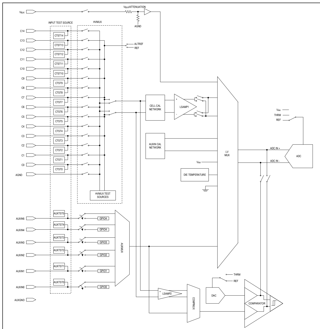
Figure 3. ADES1754/ADES1755/ADES1756 Analog Front-End
