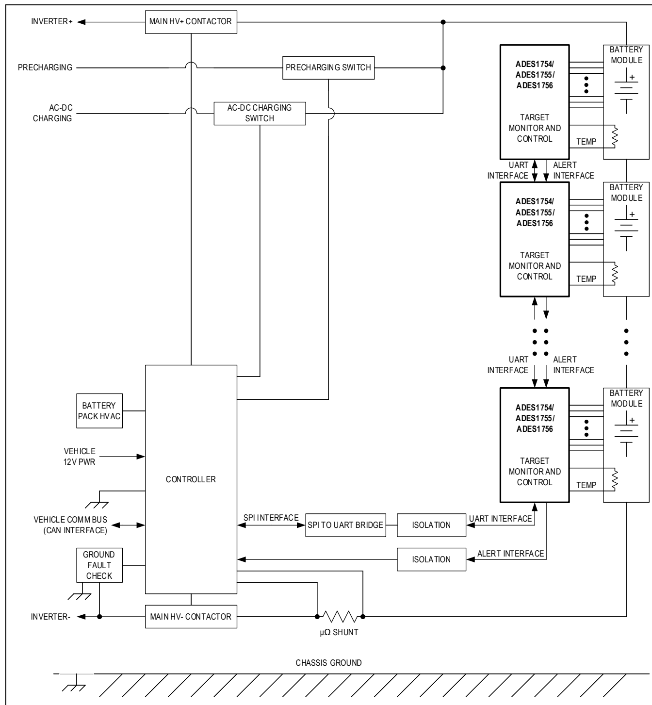
Figure 95. Daisy-Chain System
