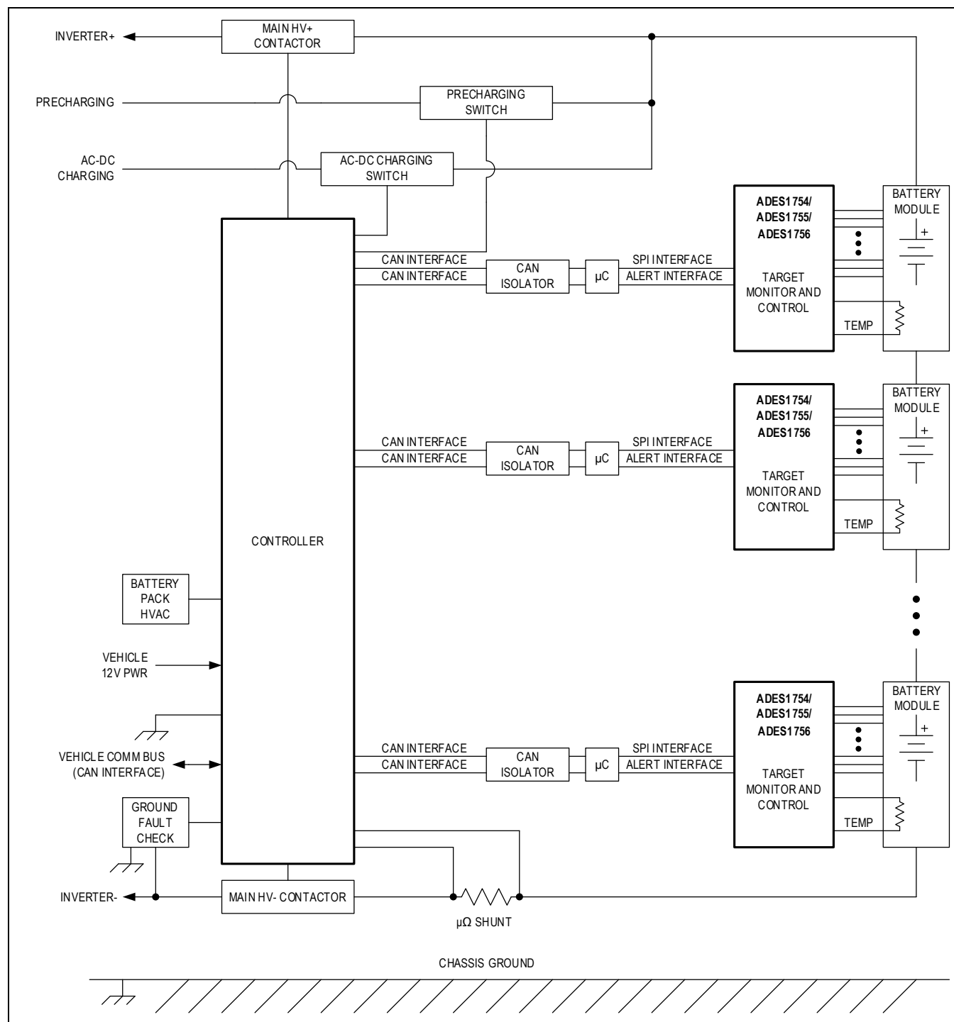
Figure 96. Distributed System
