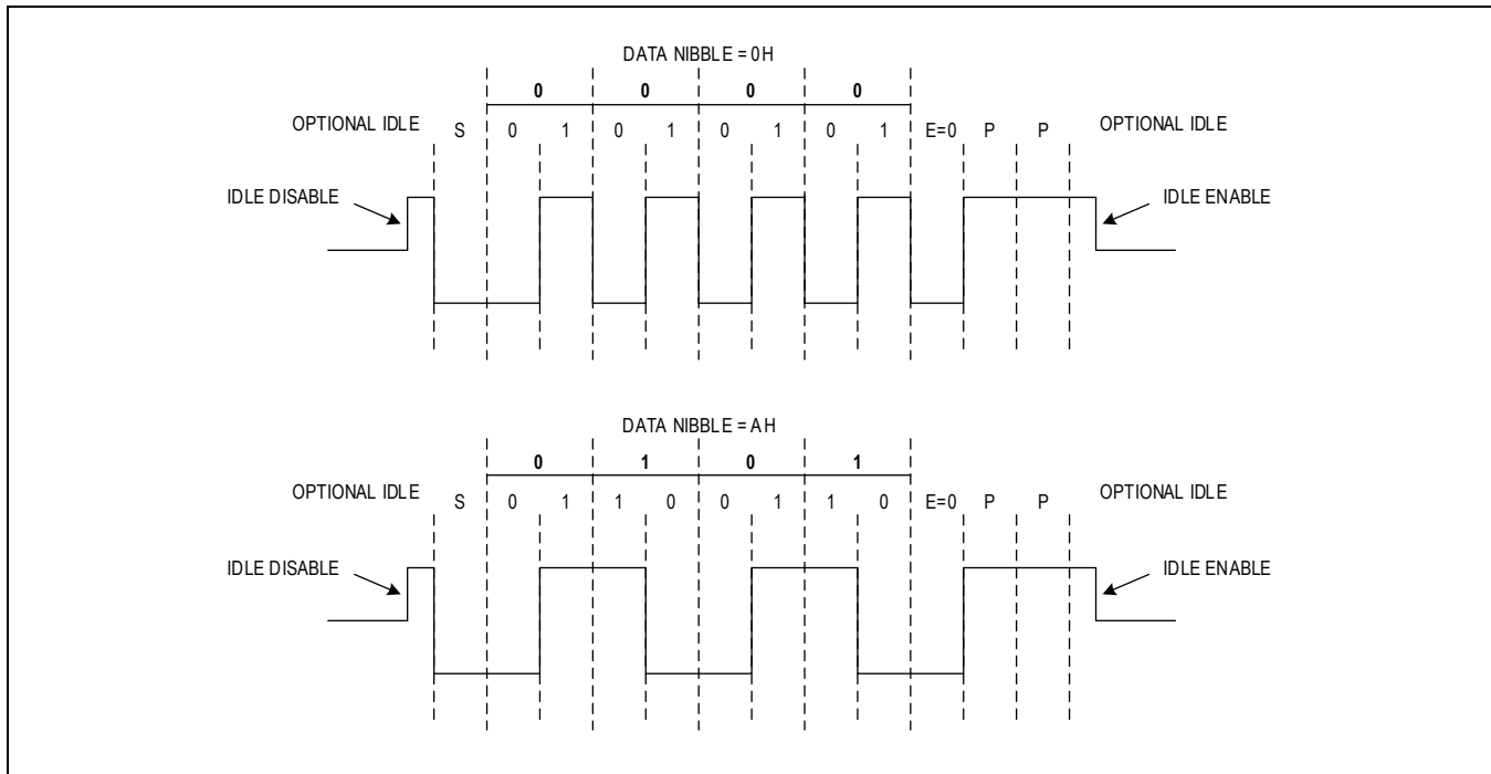
Figure 56. Data Characters
