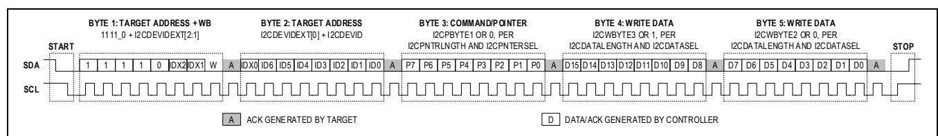
Figure 62. I 2 C Write Mode Transaction Example—10-Bit Address, I2C10BIT = 1
