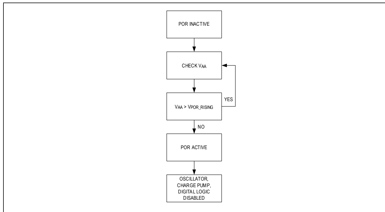
Figure 13. Shutdown Sequence
