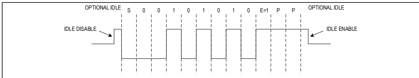
Figure 57. Stop Character
