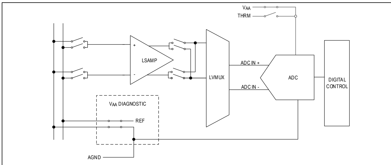
Figure 73. V_{AA} Diagnostic
