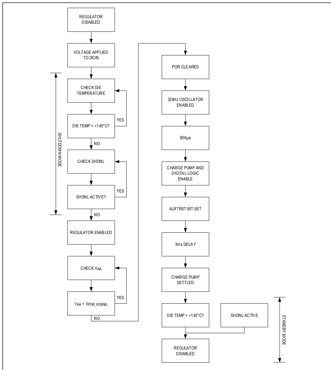
Figure 12. Power-On Sequence
