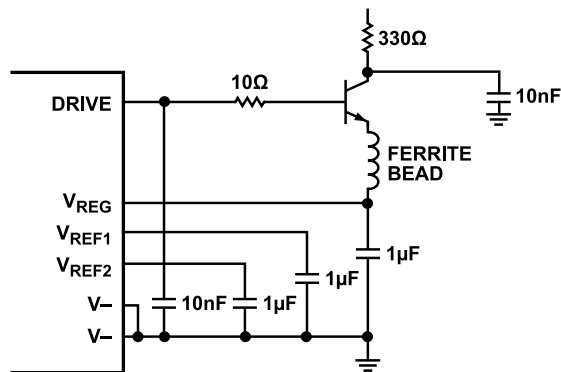
Figure 37. V_{\text{REG}} Power Source Using NPN Pass Transistor
