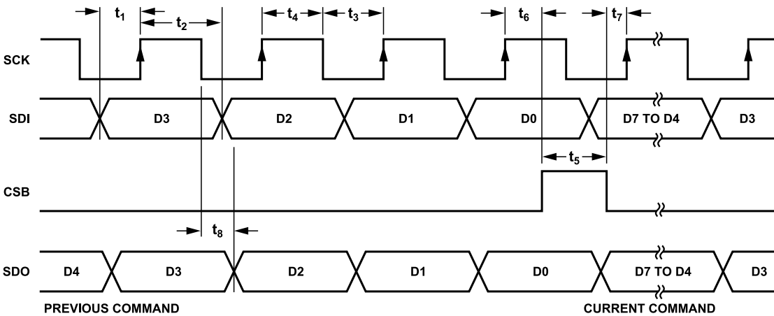
Figure 27. Timing Diagram of 4-Wire SPI
