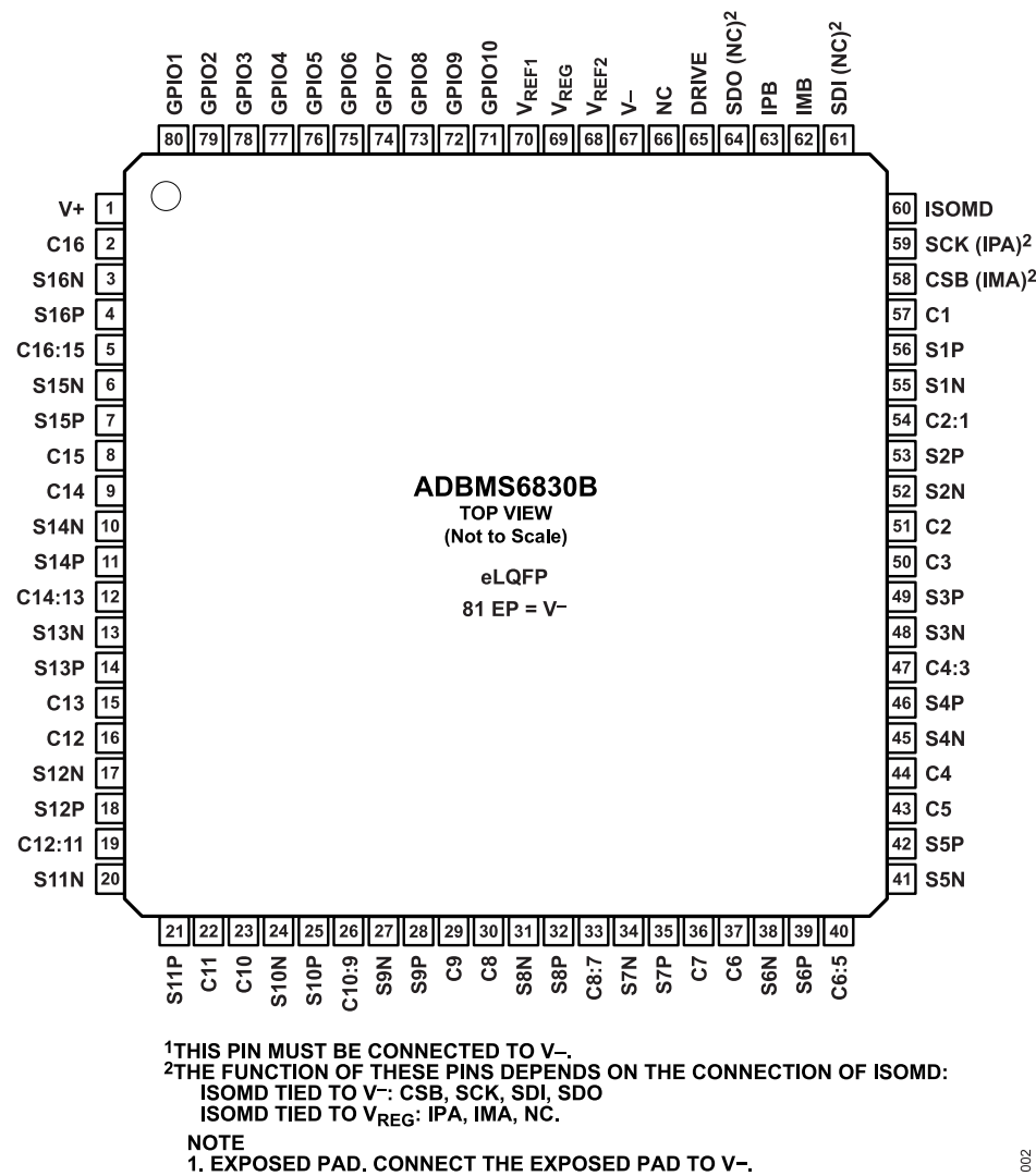
Figure 3. Pin Configuration, 80-Lead LQFP_EP
