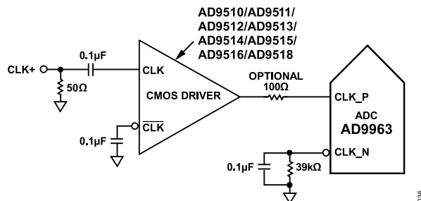
Figure 67. Single-Ended 1.8 V CMOS Sample Clock
