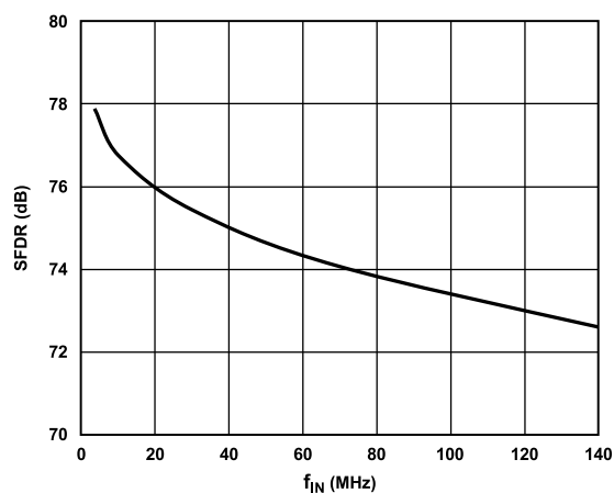
Figure 29. AD9963 100 MSPS Single Tone AC
