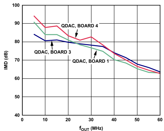
Figure 26. Intermodulation Distortion vs. f_{OUT} , TXVDD = 3.3 V , Full-Scale Current = 2 mA, Board-to-Board Variation
