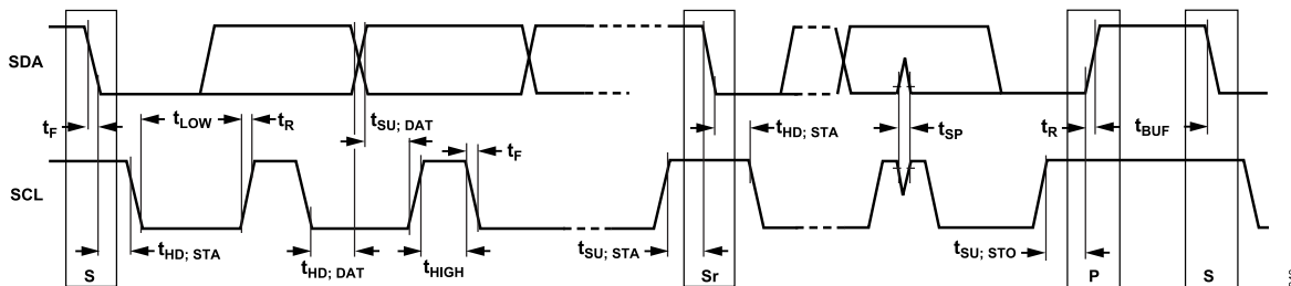
Figure 48. I 2 C Serial Port Timing
