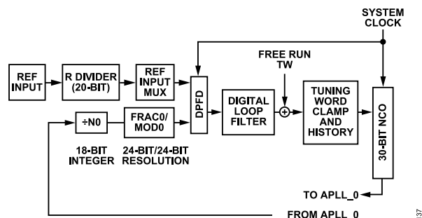
Figure 31. DPLL_0 Core
