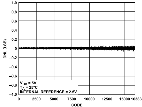
Figure 16. AD5695R DNL
