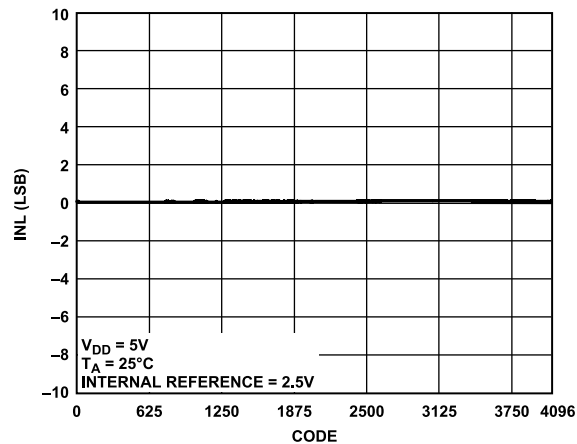
Figure 14. AD5694R INL
