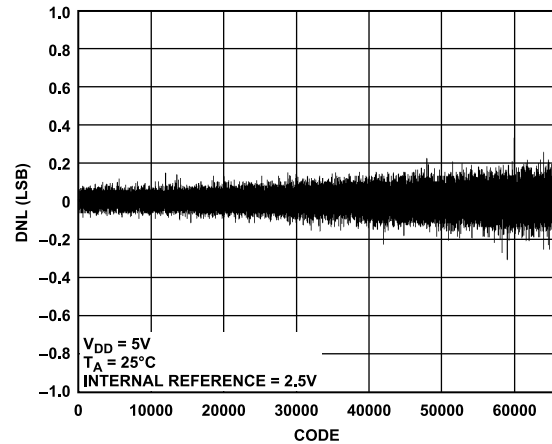
Figure 15. AD5696R DNL
