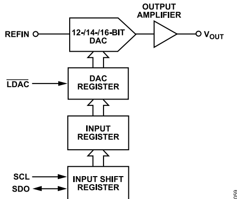
Figure 53. Simplified Diagram of Input Loading Circuitry for a Single DAC
