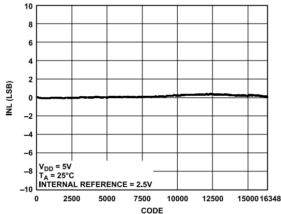
Figure 13. AD5695R INL
