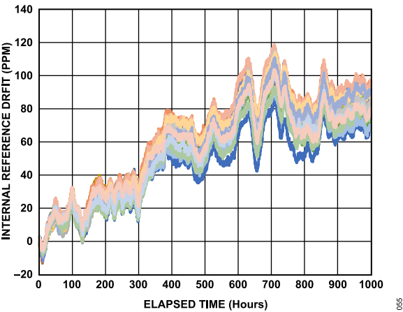
Figure 55. Reference Drift Through to 1000 Hours
