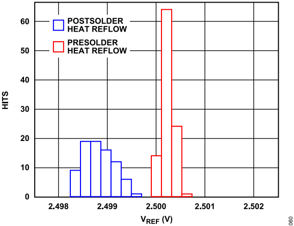
Figure 54. SHR Reference Voltage Shift
