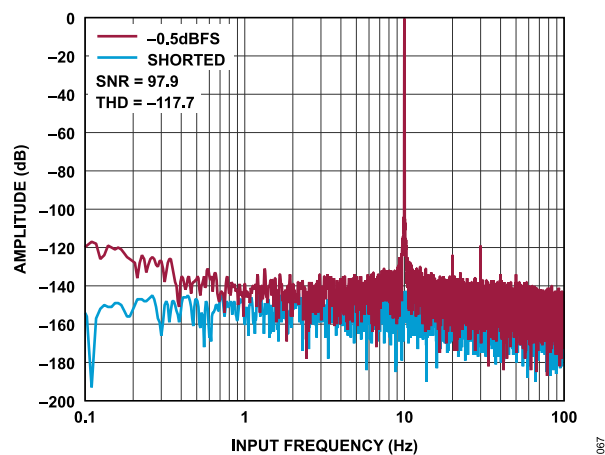
Figure 65. FFT, -0.5 dBFS vs. Shorted Inputs, 10 Hz Input Tone, \text{Sinc}^3 Filter, ODR = 240 SPS, Gain = 1, Internal Reference
