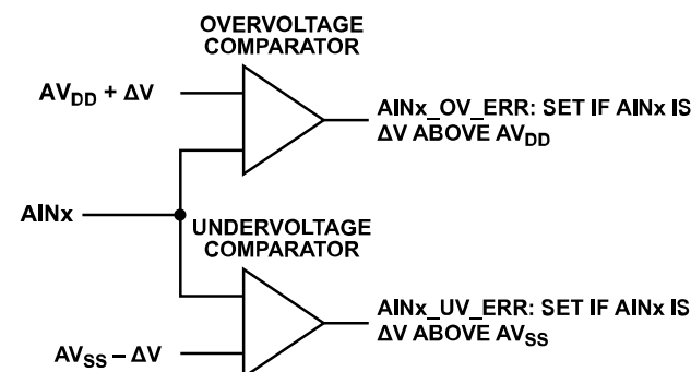
Figure 93. Analog Input Overvoltage/Undervoltage Monitors
