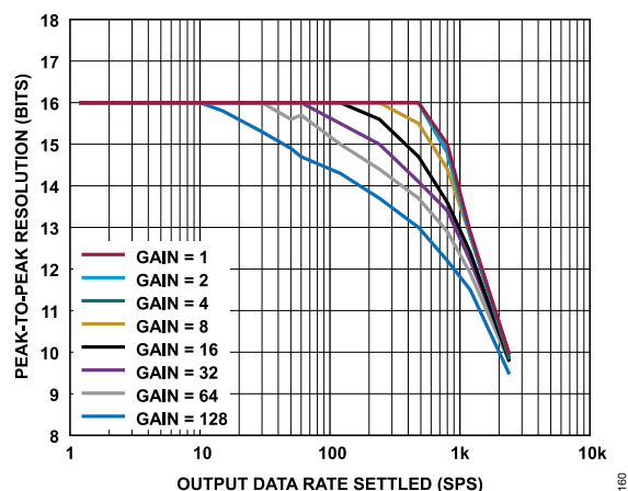
Figure 61. Peak-to-Peak Resolution vs. Output Data Rate (Settled) for Various Gains (Sinc 3 Filter)
