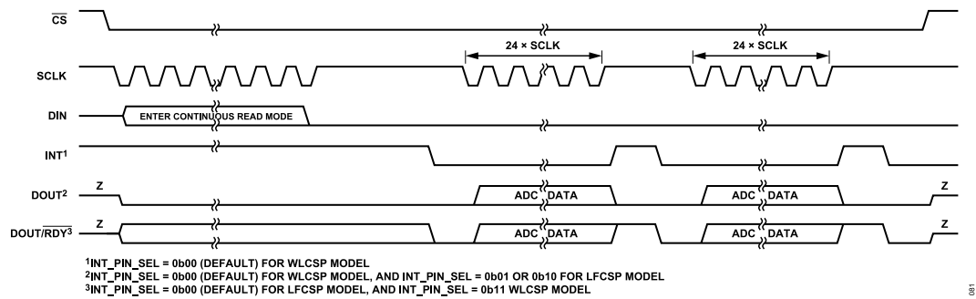
Figure 78. Enter Continuous Read Mode Diagram (DATA_STATUS = 0)
