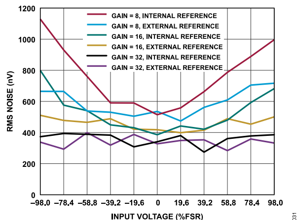
Figure 29. RMS Noise vs. Analog Input Voltage ( \text{Sinc}^3 Filter, ODR = 50 SPS, Gain = 8, Gain = 16 and Gain = 32, 2.5 V Reference)
