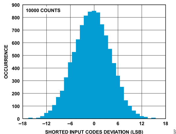
Figure 28. Noise Histogram Plot ( \text{Sinc}^4 Filter, ODR = 240 SPS, Gain = 1, Internal 1.25 V Reference)
