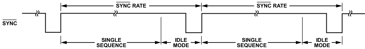
Figure 74. Example of Single Sequence + Idle by \overline{\text{SYNC}} Mode Diagram
