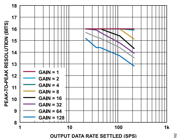
Figure 63. Peak-to-Peak Resolution vs. Output Data Rate (Settled) for Various Gains (Sinc 4 Filter)
