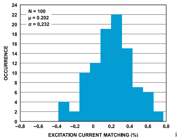
Figure 58. Excitation Current Initial Matching Histogram (100 \mu A)
