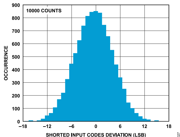
Figure 25. Noise Histogram Plot ( \text{Sinc}^3 Filter, ODR = 50 SPS, Gain = 1, Internal 2.5 V Reference)
