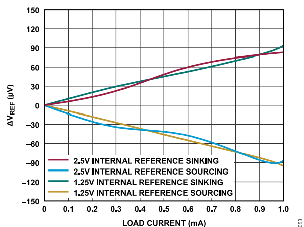
Figure 51. 1.25 V ( AV_{DD} = 1.8 V) and 2.5 V ( AV_{DD} = 3.3 V) Internal Reference Voltage vs. Load Current
