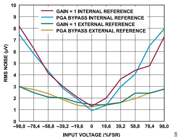
Figure 26. RMS Noise vs. Analog Input Voltage ( \text{Sinc}^3 Filter, ODR = 50 SPS, Gain = 1 and Gain = 1 with PGA Bypass, 2.5 V Reference)
