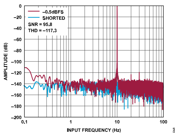
Figure 66. FFT, -0.5 dBFS vs. Shorted Inputs, 10 Hz Input Tone, \text{Sinc}^3 Filter, ODR = 240 SPS, Gain = 1, External Reference
