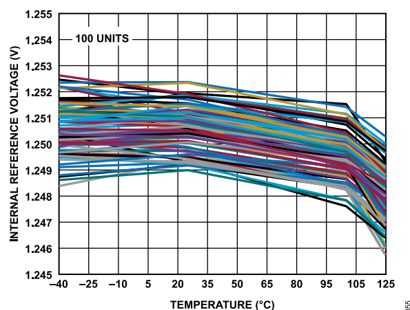
Figure 53. 1.25 V Internal Reference Voltage vs. Temperature
