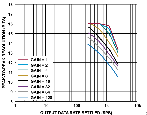
Figure 64. Peak-to-Peak Resolution vs. Output Data Rate (Settled) for Various Gains (Sinc 4 + Sinc 1 Filter)
