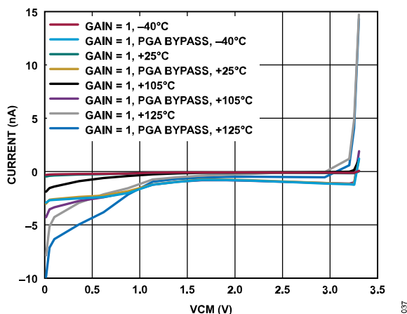
Figure 35. Absolute AINM Current vs. VCM for Various Temperatures (Gain = 1, VDIFF = 0 V)
