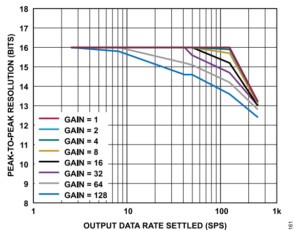
Figure 62. Peak-to-Peak Resolution vs. Output Data Rate (Settled) for Various Gains (Sinc 3 + Sinc 1 Filter)
