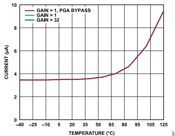
Figure 45. IOV_{DD} Current vs. Temperature
