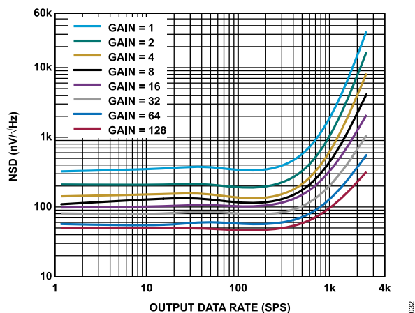
Figure 30. NSD vs. Output Data Rate for Various Gains ( \text{Sinc}^3 Filter, External 2.5 V Reference)
