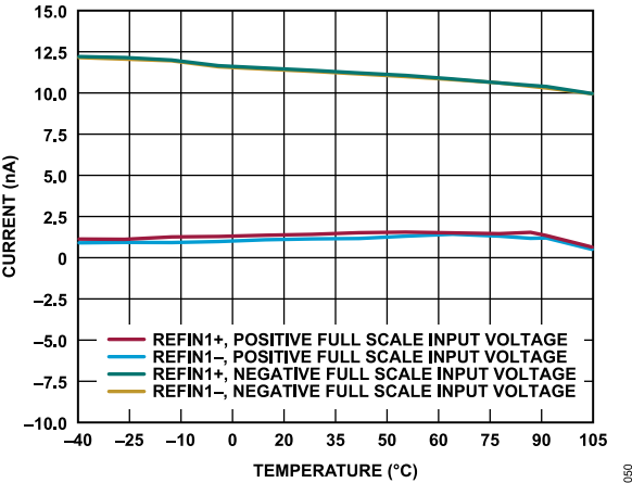
Figure 48. Reference Input Current vs. Temperature (Reference Buffer Bypass, External 2.5 V Reference)
