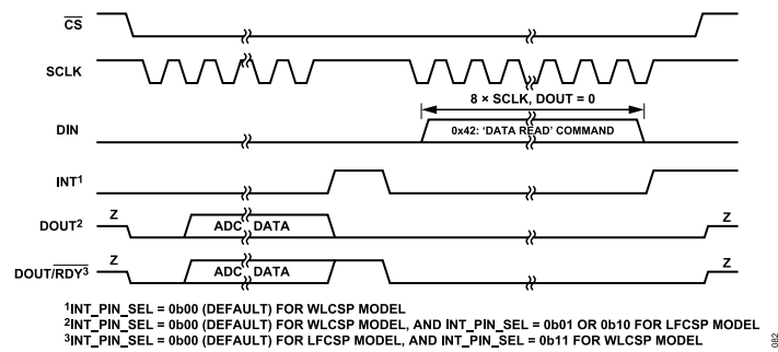
Figure 79. Exit Continuous Read Mode Diagram (CRC Disabled)
