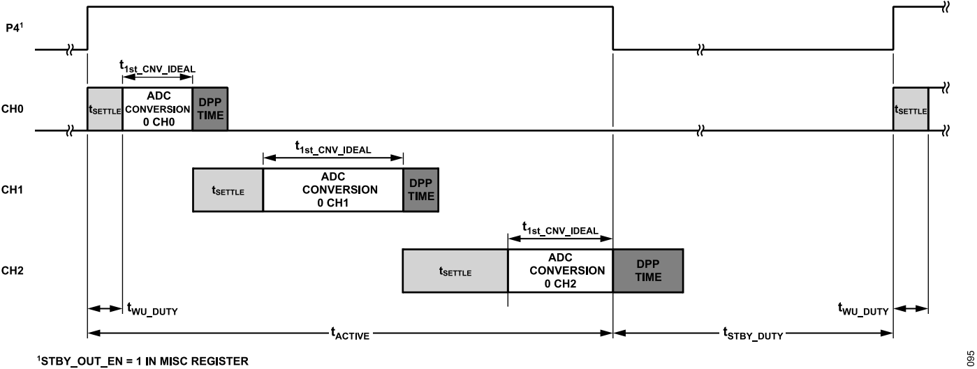
Figure 90. Example of Autonomous Duty Cycling Mode
