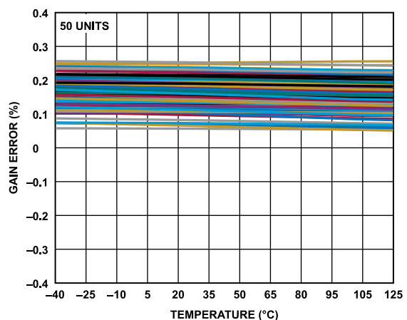
Figure 17. Gain Error vs. Temperature (Gain = 8, Before Calibration)
