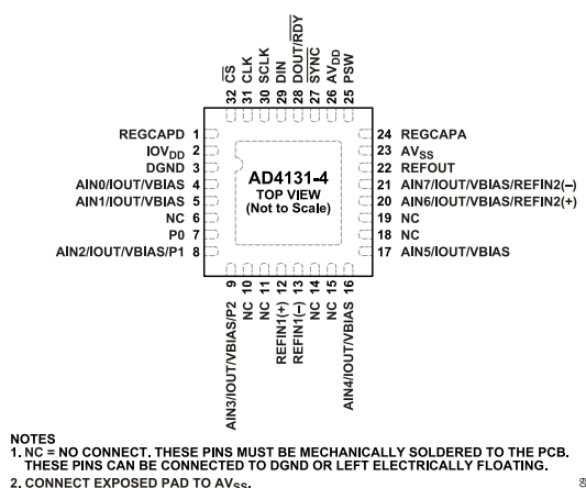
Figure 12. LFCSP Pin Configuration
