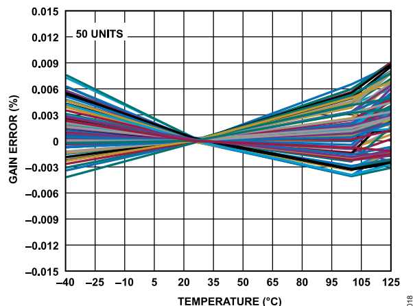
Figure 16. Gain Error vs. Temperature (Gain = 1, Factory Calibrated)
