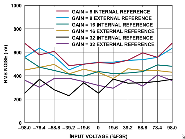
Figure 27. RMS Noise vs. Analog Input Voltage ( \text{Sinc}^3 Filter, ODR = 50 SPS, Gain = 8, Gain = 16 and Gain = 32, 1.25 V Reference)
