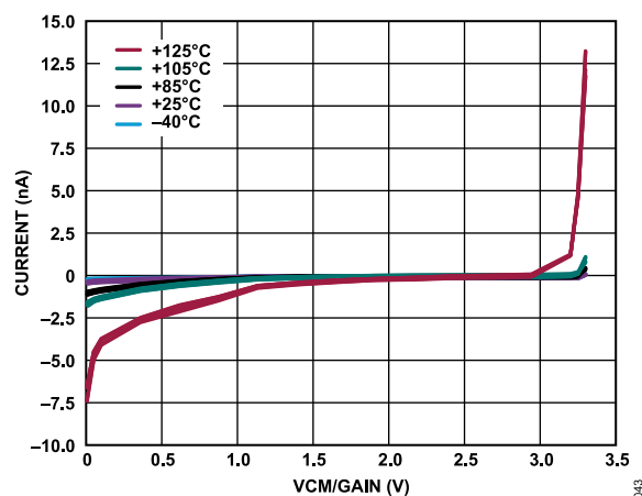
Figure 41. Absolute AINM Current vs. VCM/Gain for Various Temperatures (Gain = 2 to 128, VDIFF = 0 V)
