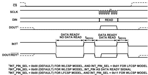
Figure 9. Data Ready High Time when Data Ready is Initially Low and the Next Conversion is Available
