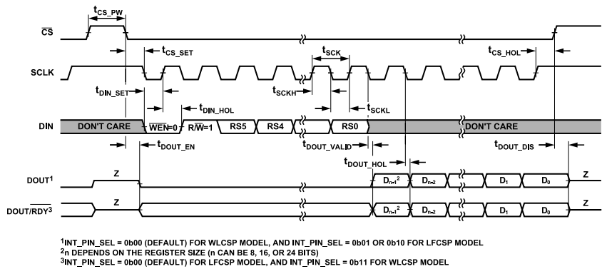
Figure 8. Read Cycle Timing Diagram, 4-Wire Mode (CSB_EN Bit Set to 1)
