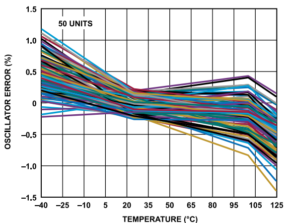
Figure 24. Internal Oscillator Error vs. Temperature
