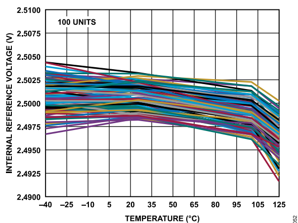
Figure 50. 2.5 V Internal Reference Voltage vs. Temperature
