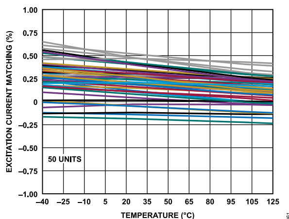
Figure 59. Excitation Current Matching vs. Temperature (100 \mu A)
