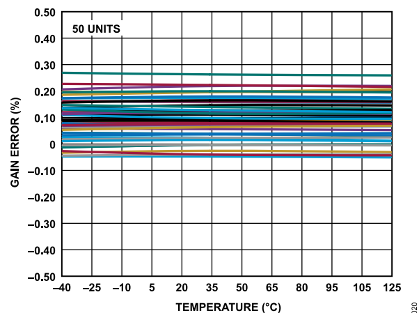
Figure 18. Gain Error vs. Temperature (Gain = 32, Before Calibration)
