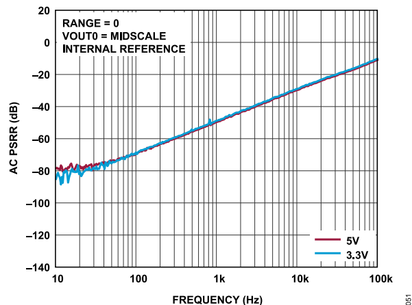
Figure 50. MUX_OUT AC PSRR vs. Frequency
