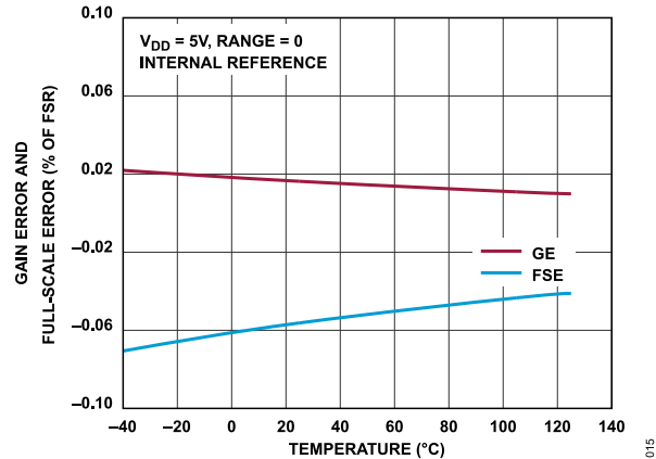
Figure 15. Gain Error and Full-Scale Error vs. Temperature
