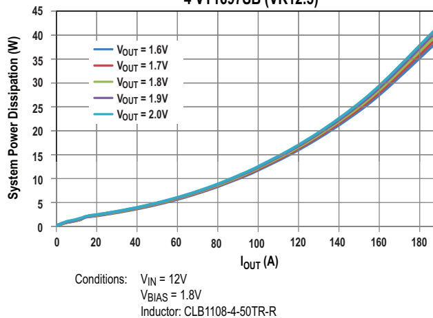
System Power Dissipation vs. Load Current 4 VT1697SB (VR12.5)
