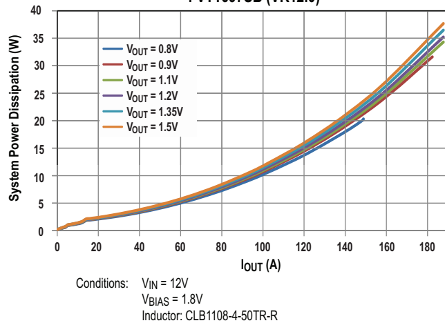
System Power Dissipation vs. Load Current 4 VT1697SB (VR12.0)
