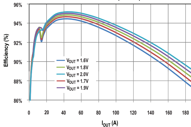
Efficiency vs. Load Current 4 VT1697SB (VR12.5)
