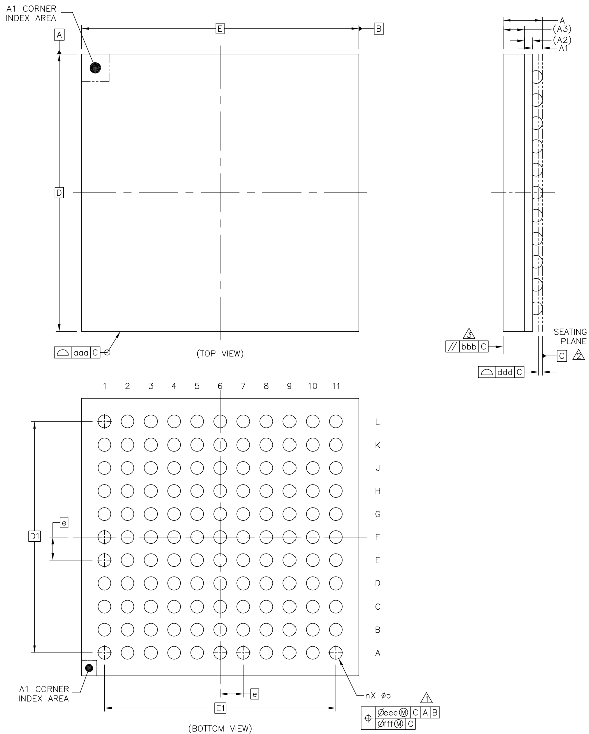
Figure 53: TMC8462A-BA package outline drawing
