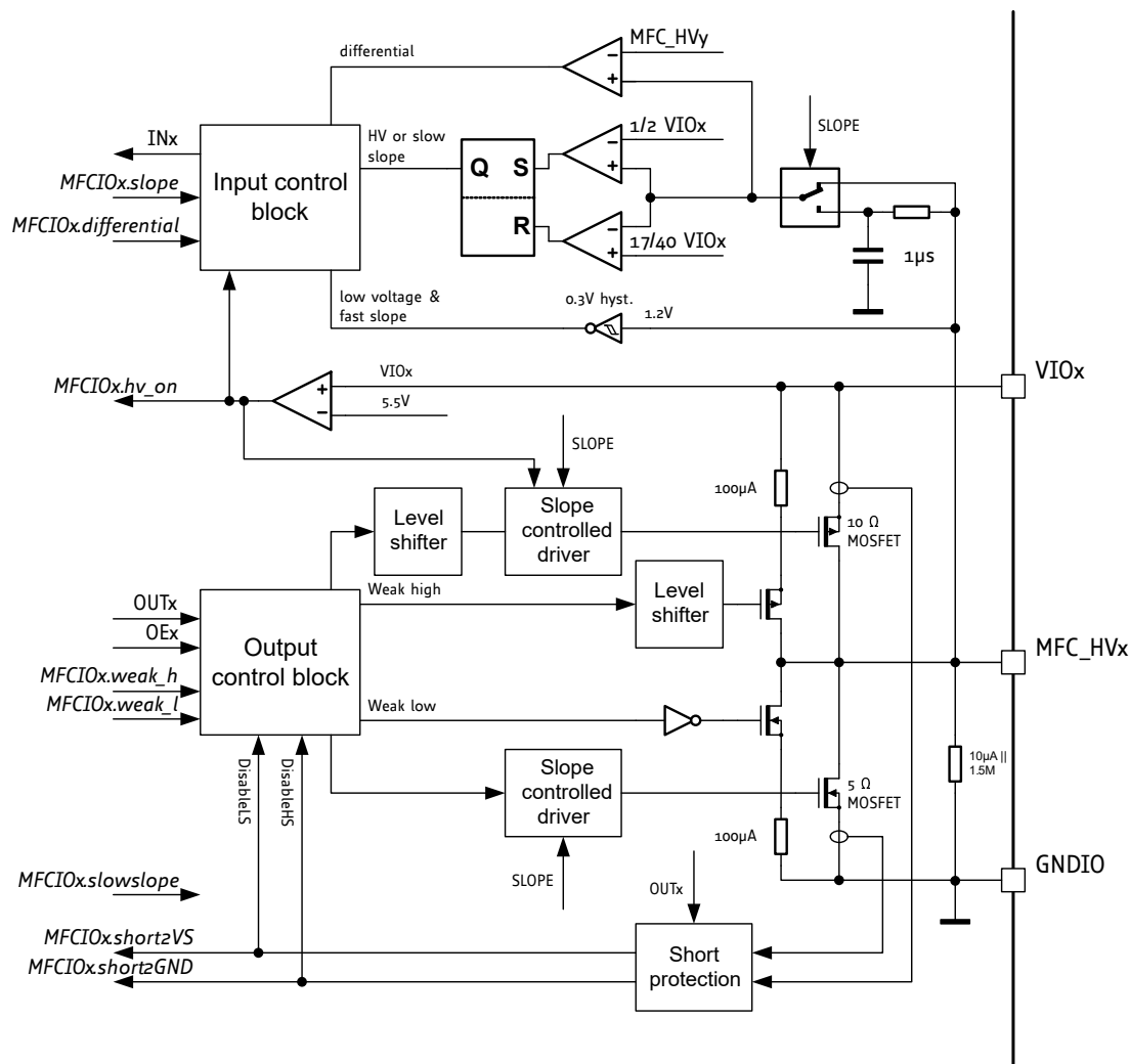
Figure 51: Schematic of multi voltage I/O port
