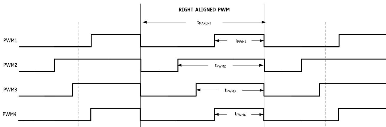
Figure 43: PWM Timing (right aligned PWM)
