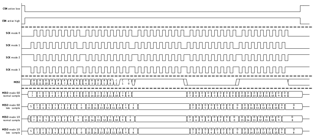
Figure 11: SPI timing example
