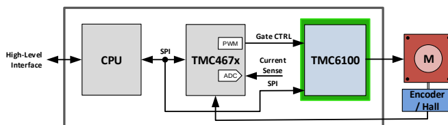
HIGH PERFORMANCE FOC SERVO DESIGN FOR PMSM
