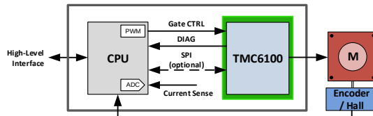
HIGH PERFORMANCE FOC SERVO DESIGN FOR PMSM
