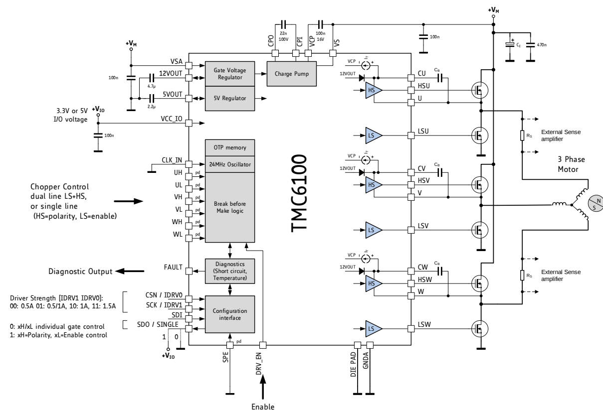
Figure 1.1 Standalone application
