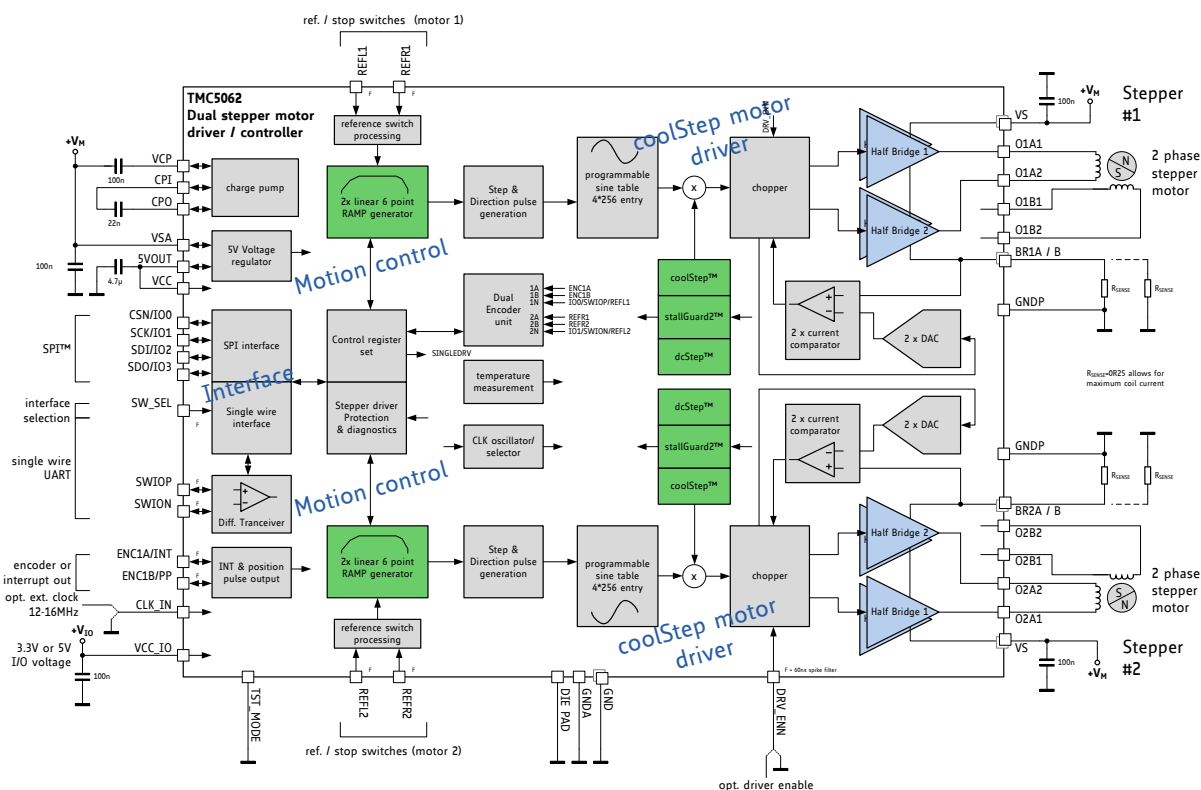
Figure 1.1 Basic application and block diagram
