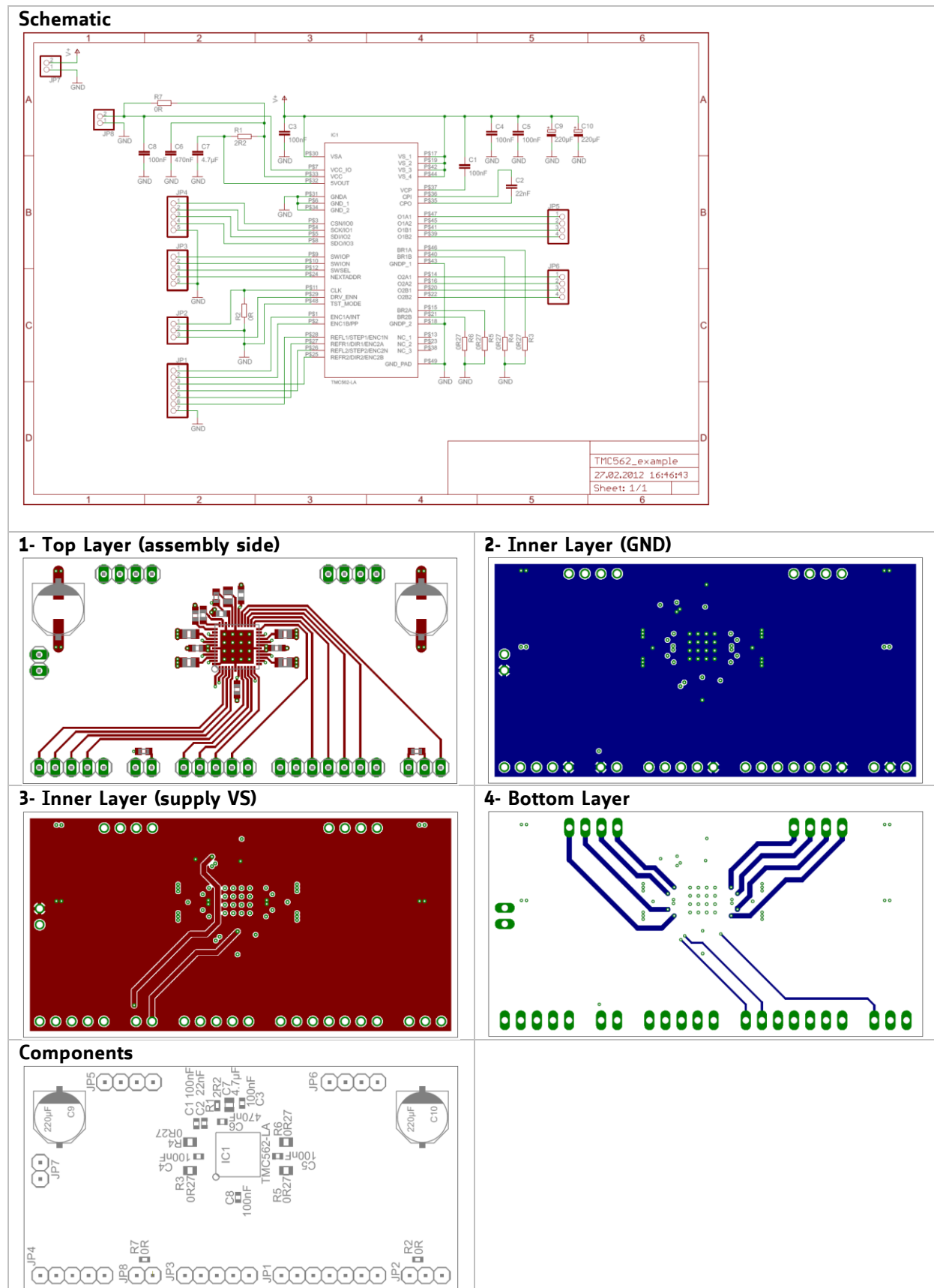
Figure 21.1 Layout example
