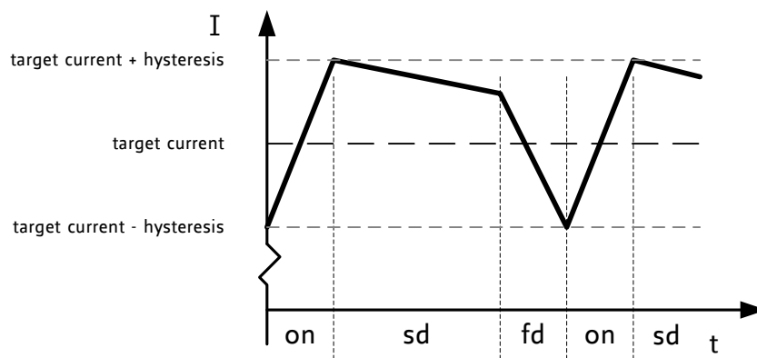
Figure 8.6 spreadCycle 3 phase chopper scheme showing the coil current within a chopper cycle
