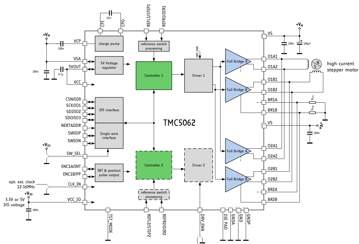
Figure 3.9 Driving a single motor with high current
