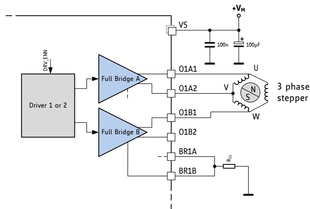
Figure 3.8 Connecting a 3-phase motor
