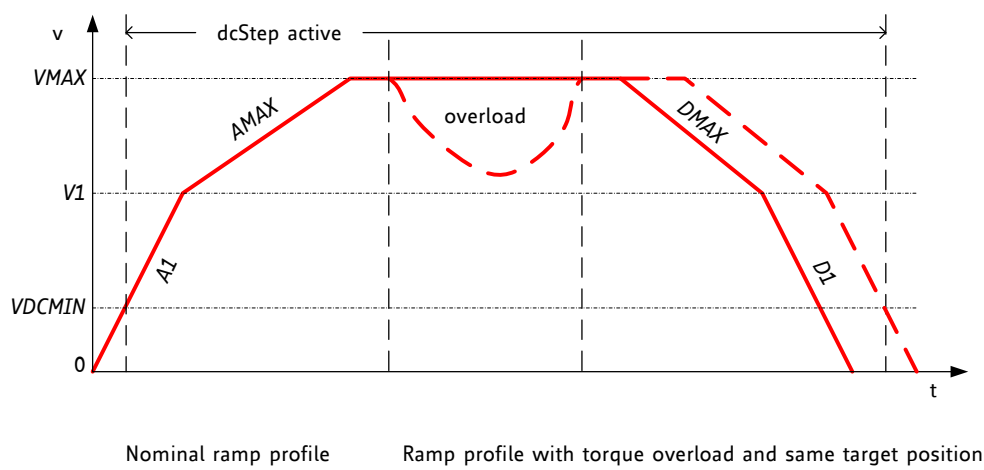
Figure 13.2 Velocity profile with impact by overload situation
