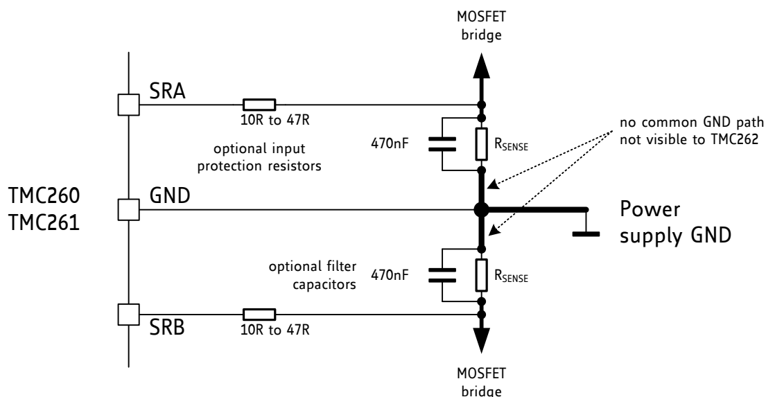
Figure 9.1 Sense resistor grounding and protection components
