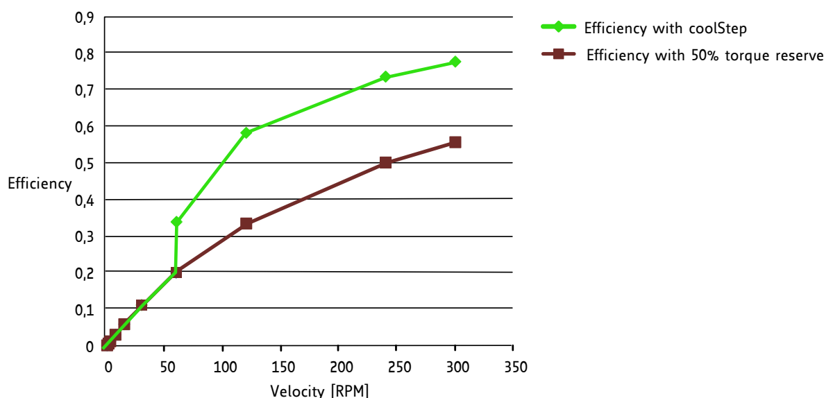
Figure 6.1 Energy efficiency example with CoolStep
