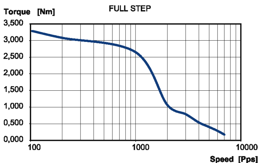
Figure 6.2: QSH8618-80-55-460 speed vs. torque characteristics
