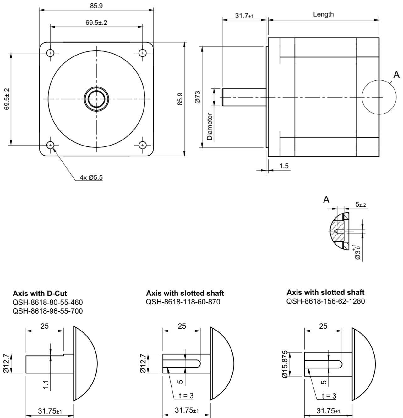
Figure 4.1: Dimensions of the QSH8618 motor family
