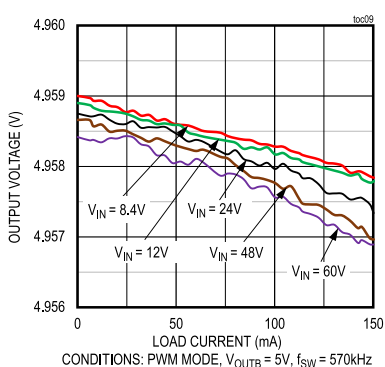
MAXM17715-MAXM17720, MAXM17721-MAXM17726 OUTPUT VOLTAGE vs. LOAD CURRENT
