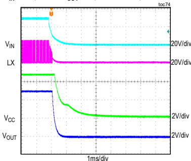
MAXM15464 SHUTDOWN THROUGH V_{IN} V_{IN} = 24V , FIXED V_{OUT} = 5V , FULL LOAD, PWM MODE
