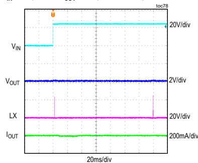
MAXM15463 OUTPUT SHORT DURING STARTUP V_{IN} = 24V , FIXED V_{OUT} = 3.3V , FULL LOAD, PWM MODE
