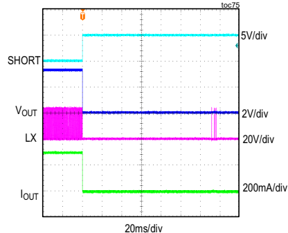
MAXM15462 OUTPUT SHORT IN STEADY STATE V_{IN} = 24V , ADJUSTABLE V_{OUT} = 3.3V , FULL LOAD, PWM MODE
