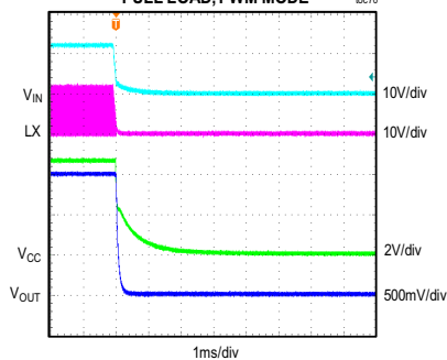
MAXM15067 SHUTDOWN THROUGH V_{IN}
