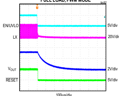
MAXM15065 SHUTDOWN THROUGH ENABLE
