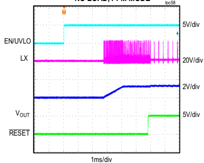
MAXM15067 STARTUP THROUGH ENABLE (2V PREBIAS)
