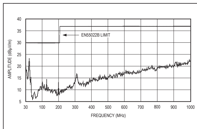
Figure 2. EMI Performance
