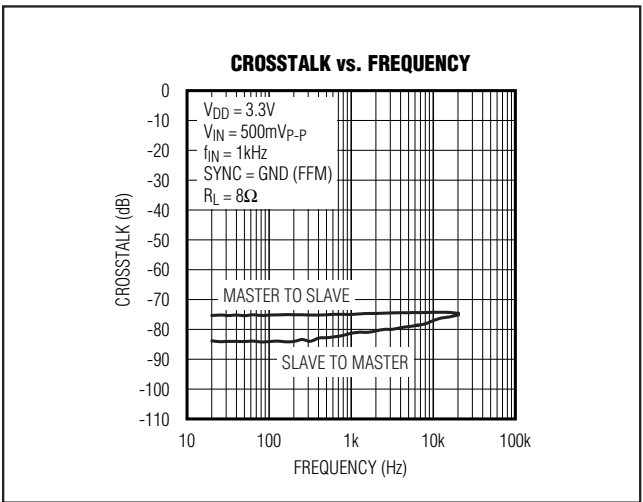
Figure 8. Master-Slave Crosstalk
