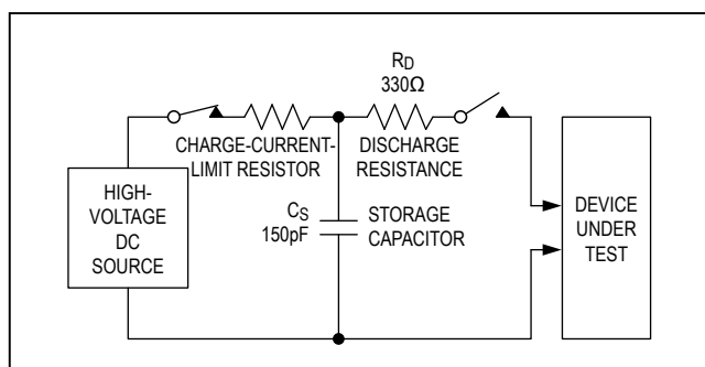
Figure 20. IEC 61000-4-2 Contact Discharge ESD Test Circuit
