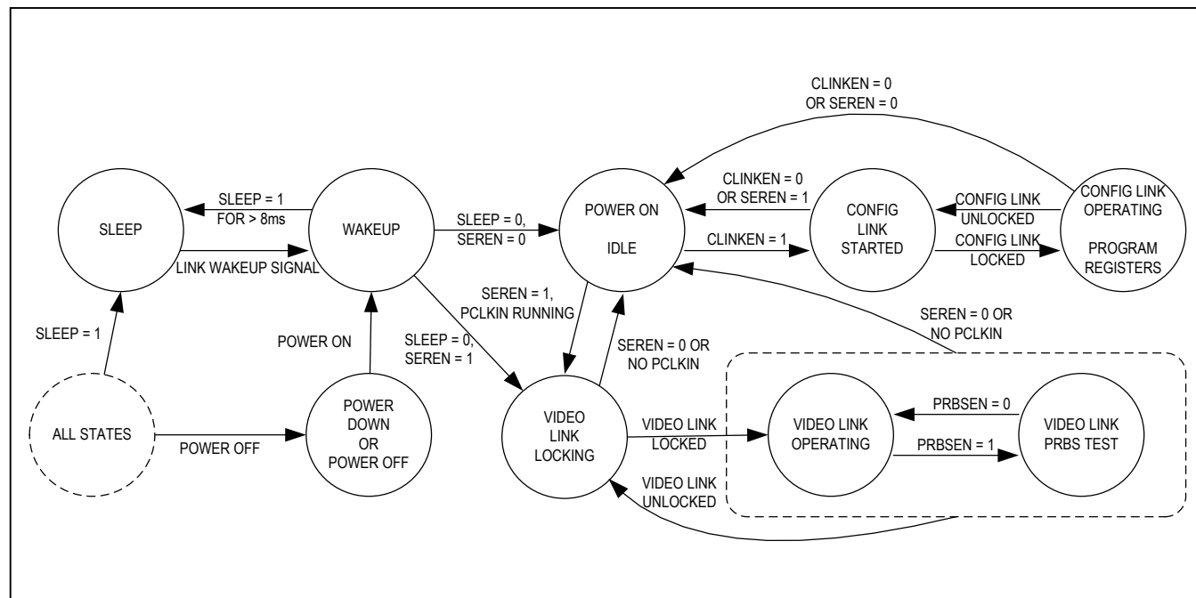
Figure 17. State Diagram
