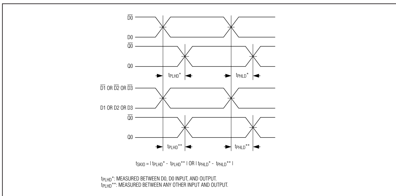
Figure 6. Input-to-Output Skew ( t_{SKIO} ) Definition
