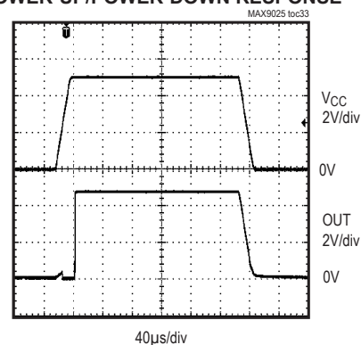
POWER-UP/POWER-DOWN RESPONSE
