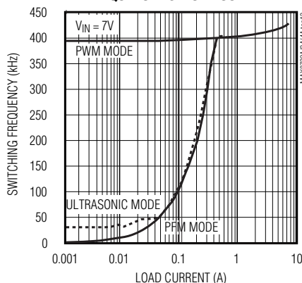
MAX8732A 3.3V OUTPUT SWITCHING FREQUENCY vs. LOAD CURRENT
