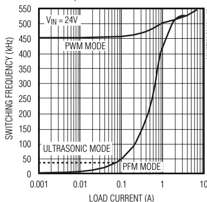
MAX8732A 3.3V OUTPUT SWITCHING FREQUENCY vs. LOAD CURRENT
