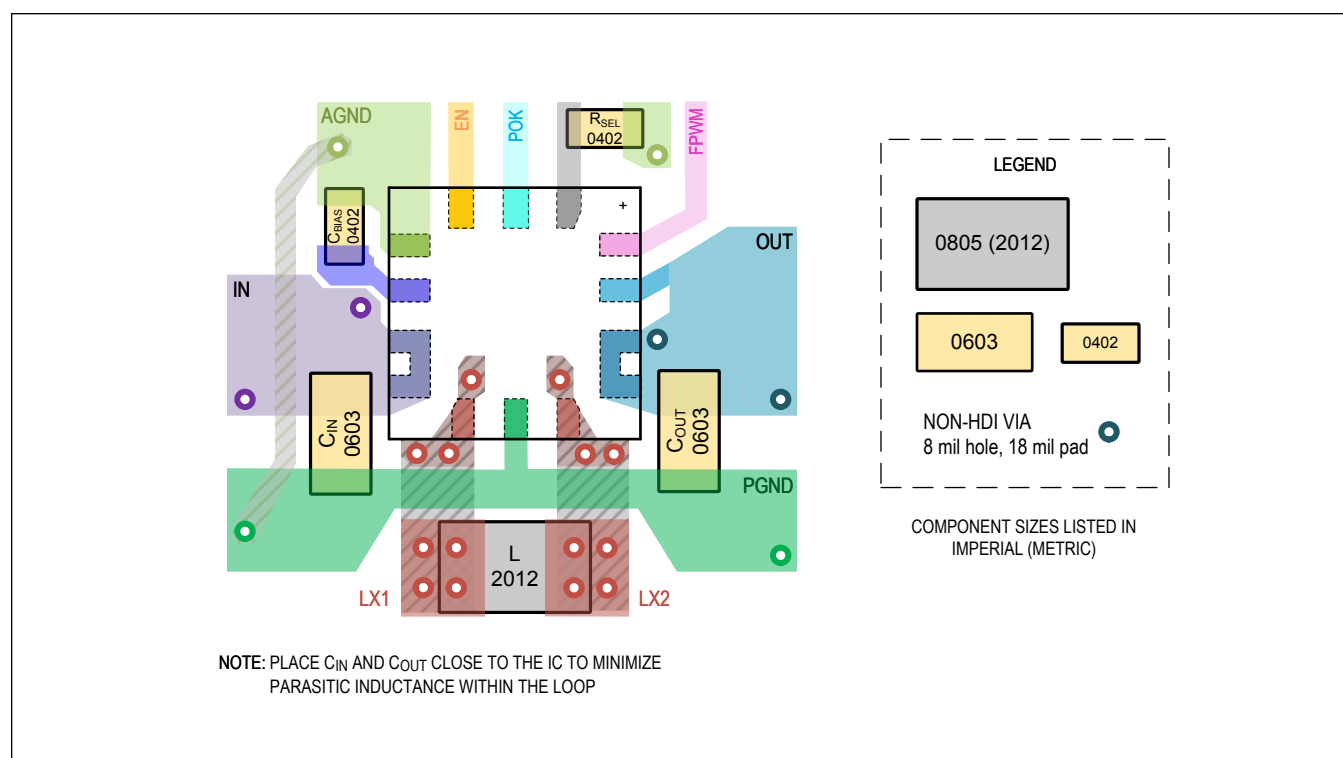
Figure 5. PCB Layout Example (FC2QFN—B and D Options)
