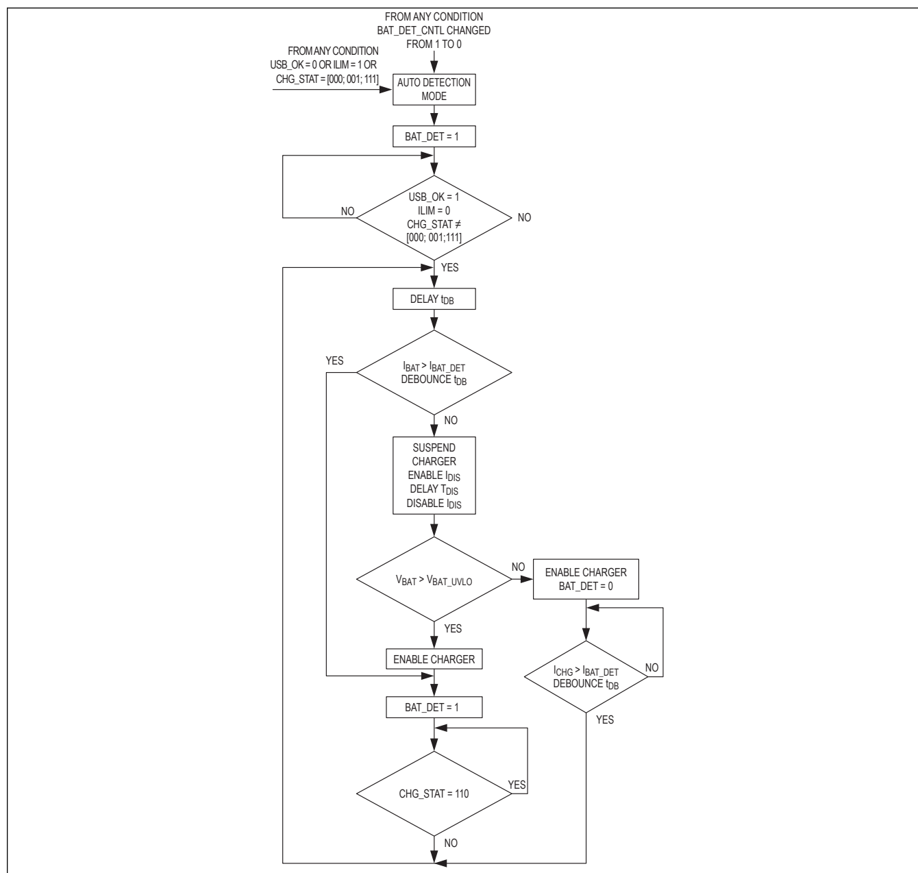
Figure 14. Battery Present Flow Chart
