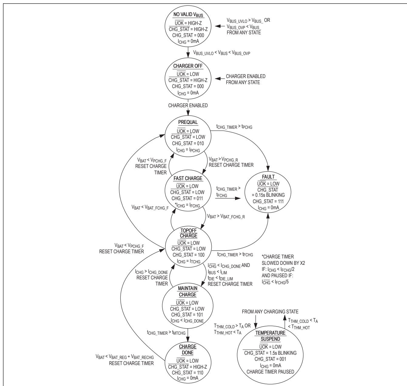
Figure 12. Charger State Diagram
