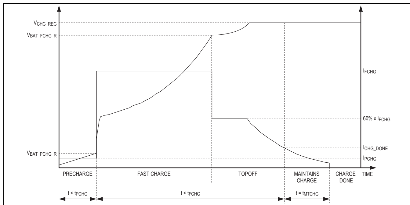
Figure 11. Charge Profile
