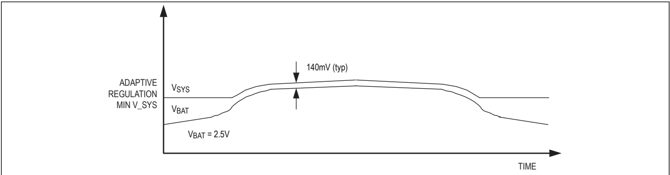
Figure 10. SYS Regulation
