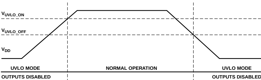
Figure 5. UVLO Function
