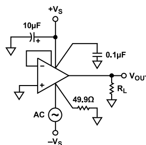
Figure 50. Negative Power Supply Rejection
