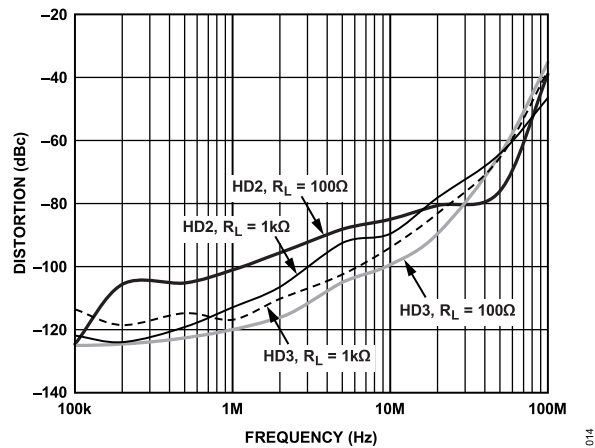
Figure 15. Distortion vs. Frequency for Various Loads, V_{OUT} = 2\text{ V p-p}
