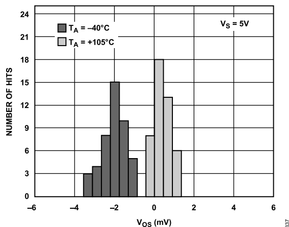
Figure 37. Input Offset Voltage Histogram over Temperature ( V_S = 5\text{ V} ), SOIC Only
