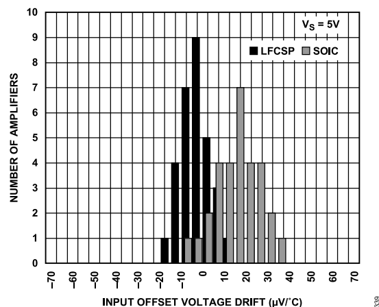
Figure 42. Input Offset Voltage Drift Histogram ( V_S = 5V )
