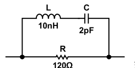
Figure 61. RLC Circuit
