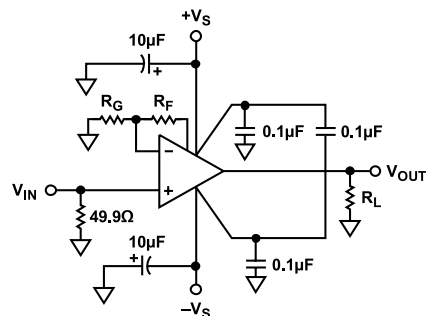
Figure 49. Noninverting Gain Configuration
