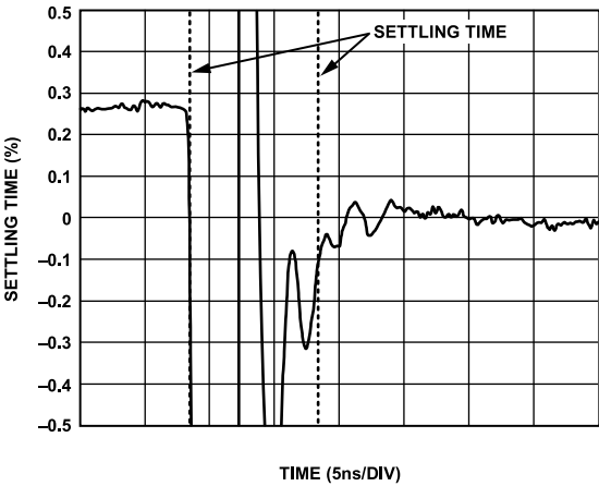
Figure 24. 0.1% Short-Term Settling Time
