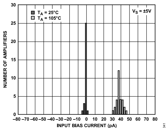
Figure 40. Input Bias Current Histogram over Temperature ( V_S = \pm 5V )
