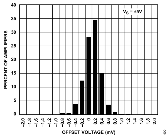
Figure 32. Input Offset Voltage Histogram ( V_S = \pm 5\text{ V} ), LFCSP Only
