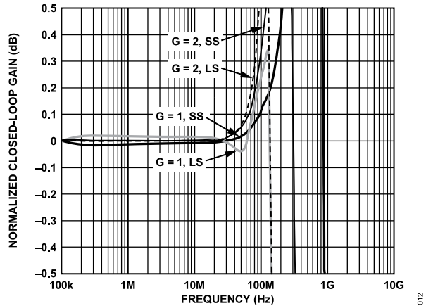
Figure 14. 0.1 dB Flatness Frequency Response vs. Gain and Output Voltage
