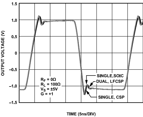
Figure 23. Large Signal Transient Response vs. Package
