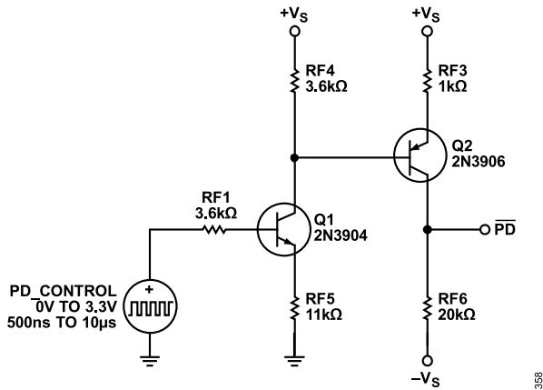
Figure 57. Power-Down Circuit
