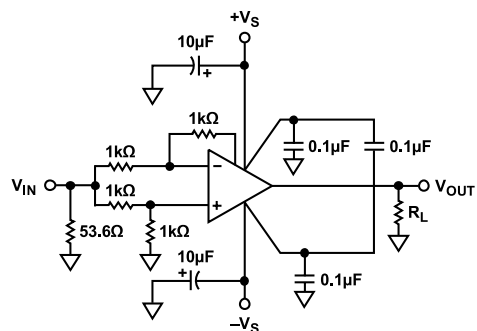
Figure 51. Common-Mode Rejection
