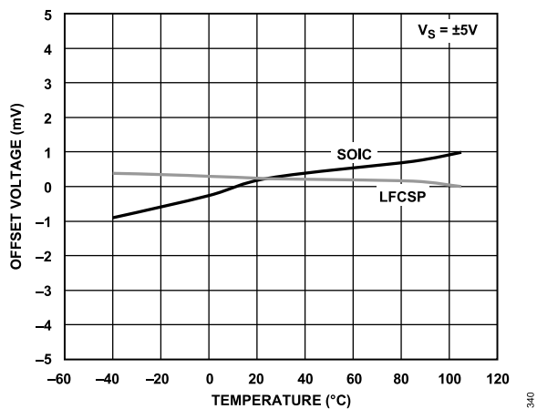
Figure 38. Offset Voltage vs. Temperature ( V_S = \pm 5V )
