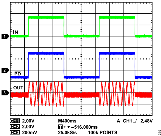
Figure 58. Power-Down Operation
