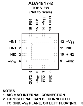
Figure 7. ADA4817-2 Pin Configuration (16-Lead LFCSP)
