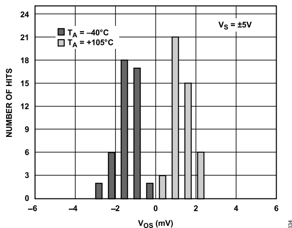
Figure 34. Input Offset Voltage Histogram over Temperature ( V_S = \pm 5\text{ V} ), SOIC Only
