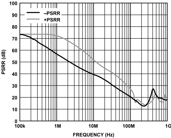
Figure 25. Power Supply Rejection Ratio (PSRR) vs. Frequency
