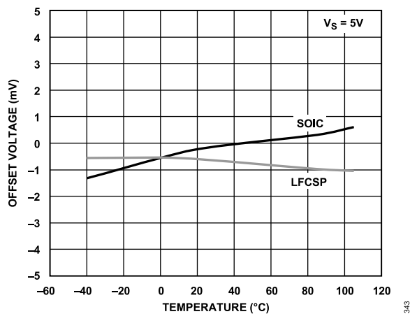
Figure 41. Offset Voltage vs. Temperature ( V_S = 5V )
