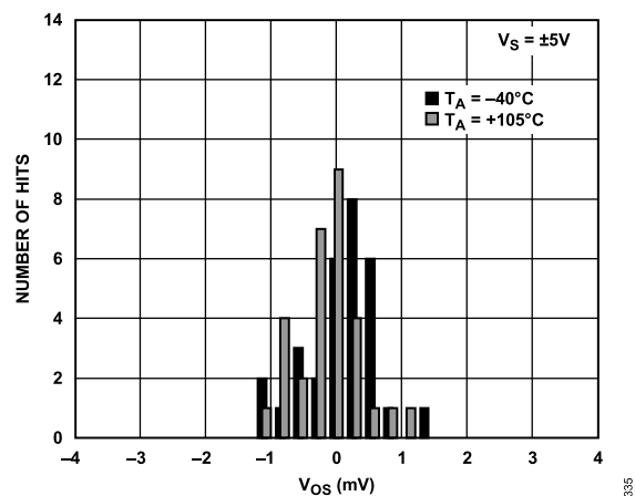
Figure 33. Input Offset Voltage Histogram over Temperature ( V_S = \pm 5\text{ V} ), LFCSP Only
