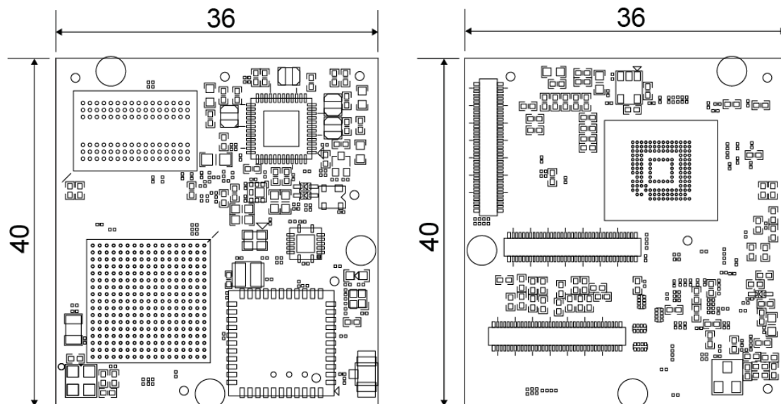
Figure 3 - PICO-IMX6UL-EMMC Dimensional Drawing
