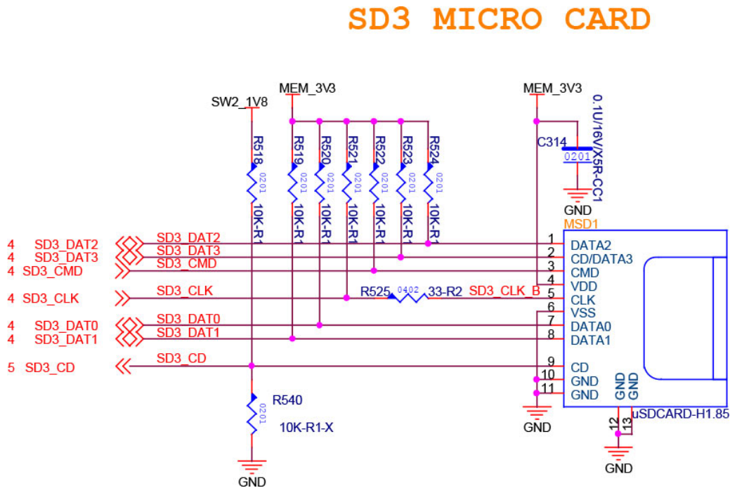
Figure 11 - SD Schematics
