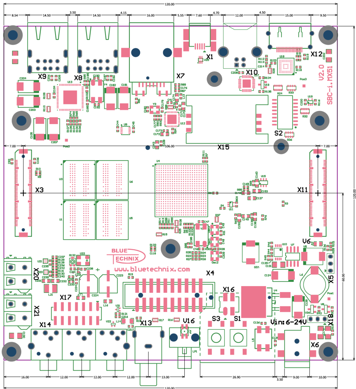
Figure 6-1: Connector dimensions
