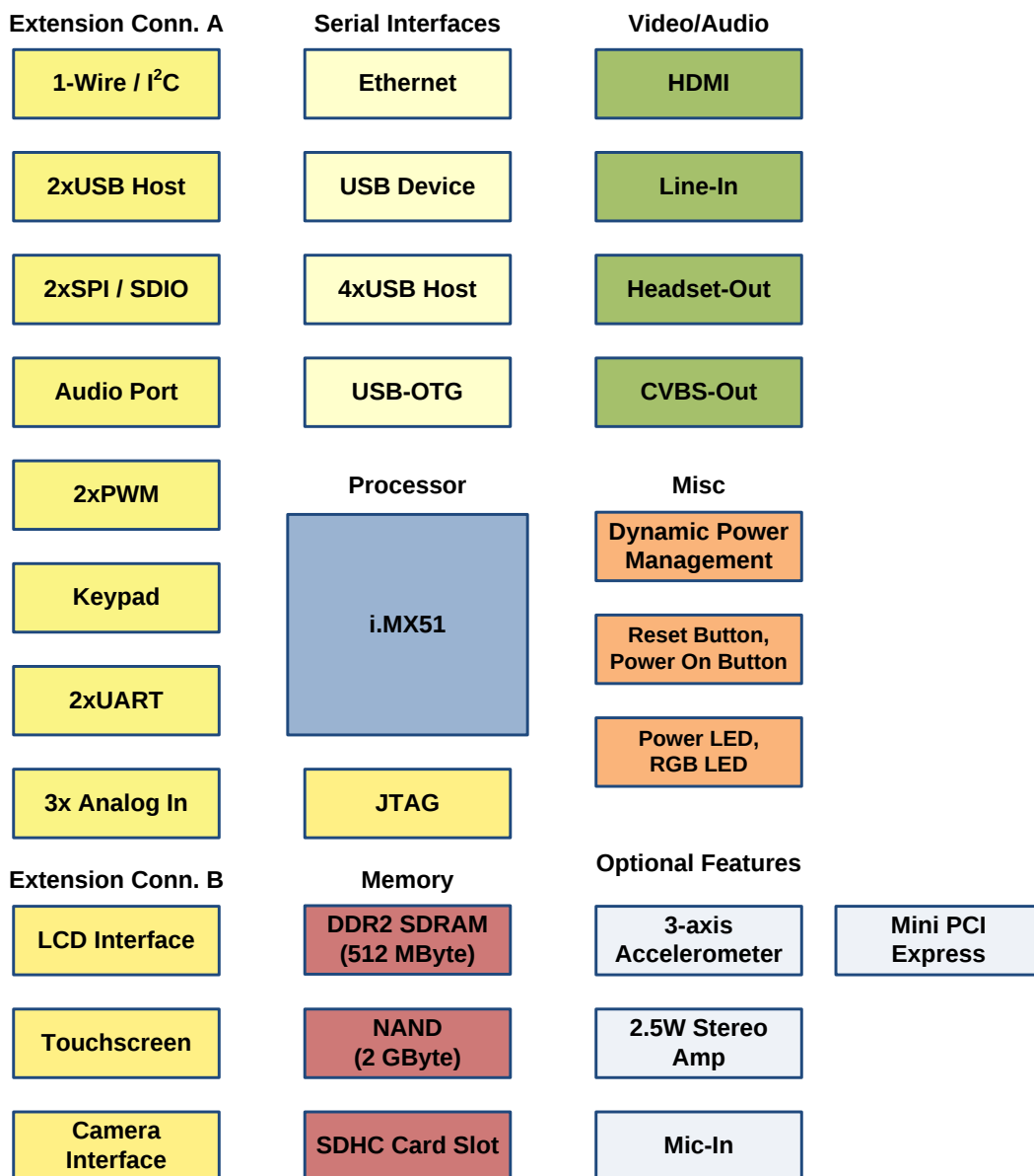
Figure 1-1: SBC-i.MX51 features
