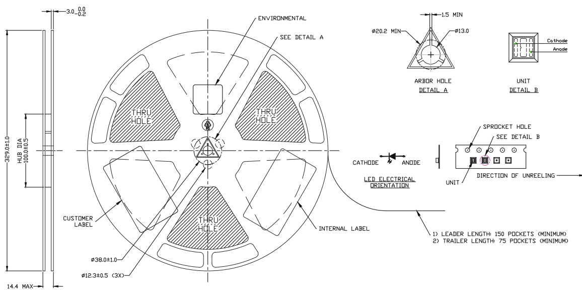
Figure 11a. Reel dimensions for LUXEON SunPlus 20 Line.
