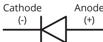
Figure 1b. Polarity of L1SP-PRPxx03500000, L1SP-RYL0003500000 and L1SP-LME0003500000.
