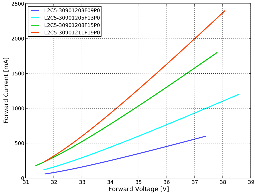
Figure 4. Typical forward current vs. forward voltage for L2C5-309012xxxxP0 at T_j=85^{\circ}\text{C} .
