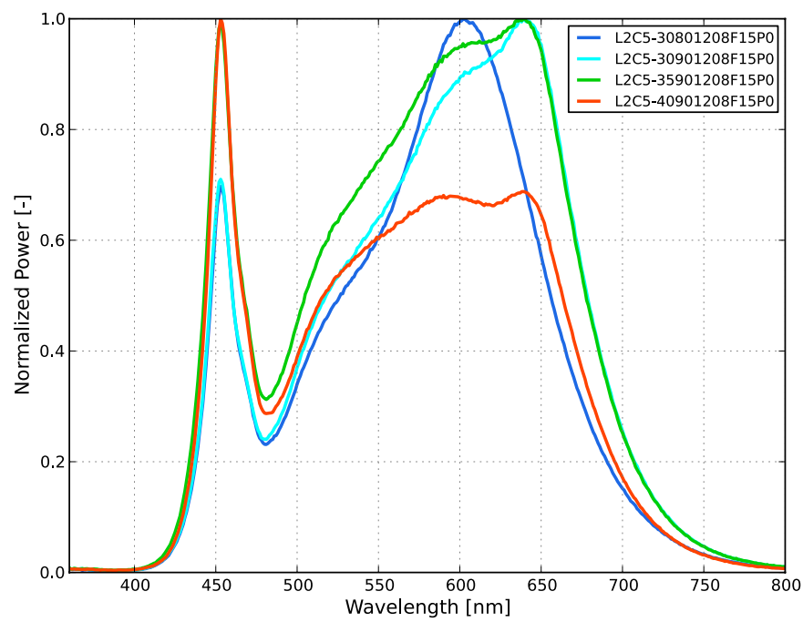
Figure 1. Typical normalized power vs. wavelength for L2C5-xxxx1208F15P0 at specified test current, T_j=85^{\circ}\text{C} .
