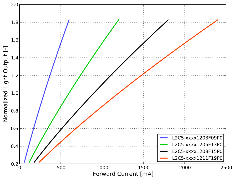
Figure 3. Typical normalized light output vs. forward current for L2C5-xxxx12xxxxP0 at T_j=85^{\circ}\text{C} .
