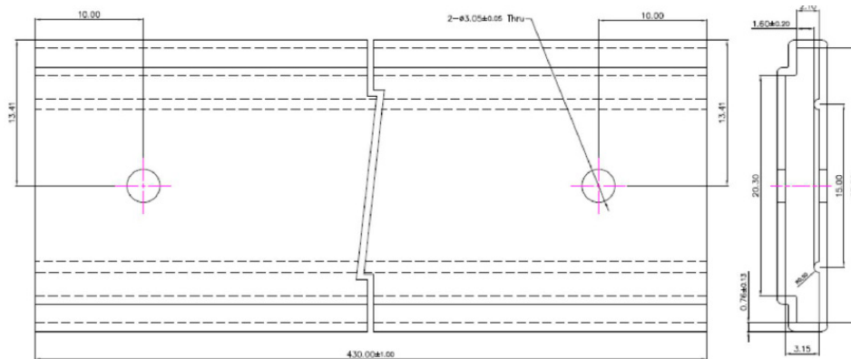
Figure 9b. Tube dimensions for L2C5-xxxx1205F13P0 and L2C5-xxxx1208F15P0.
