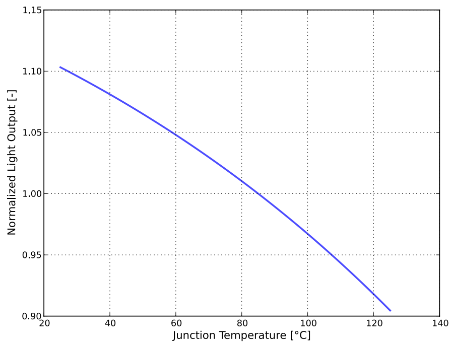
Figure 2. Typical normalized light output vs. junction temperature for L2C5-xxxx12xxxxxP0 at specified test current.
