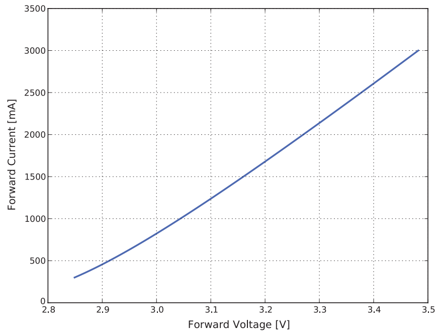
Figure 4f. Typical forward current vs. forward voltage for LUXEON Rubix Royal Blue at T_j=85^{\circ}\text{C} .
