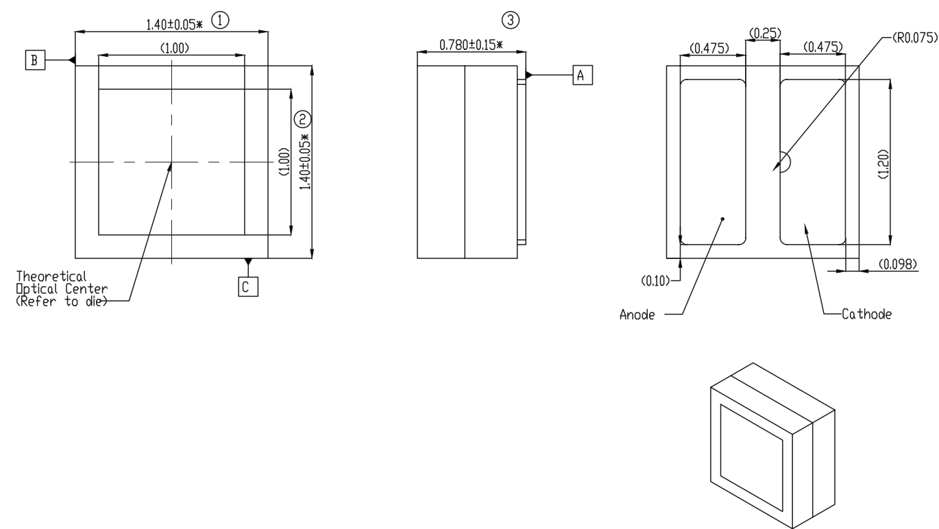
Figure 11a. Mechanical dimensions for LUXEON Rubix PC Amber, Lime, Green, Blue, Royal Blue and White Colors.
