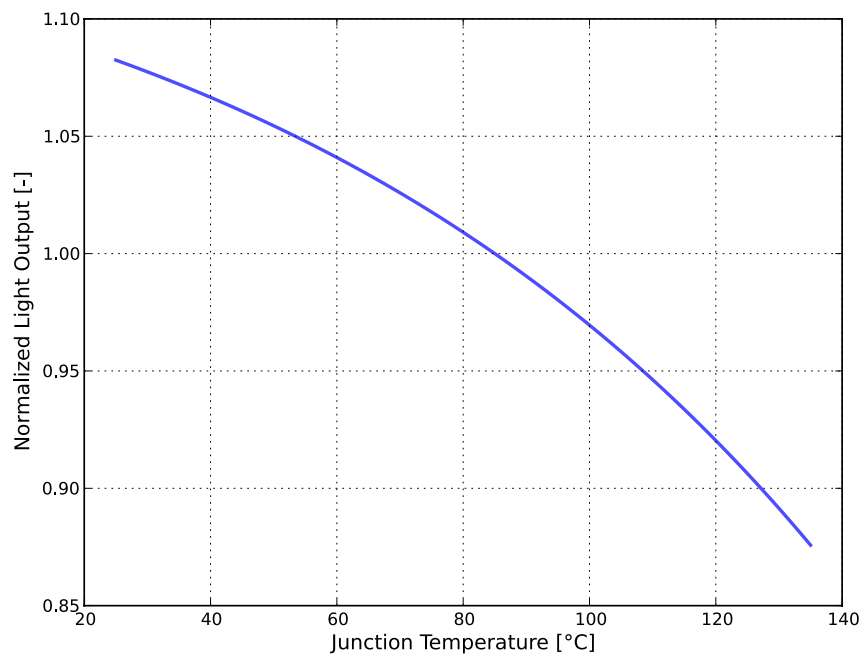
Figure 3. Typical normalized light output vs. junction temperature for LUXEON V at 1400mA, T_j = 85^\circ\text{C} .
