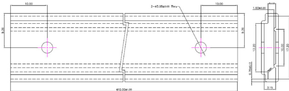
Figure 9b: Tube dimensions for L2C2-xxxxxxxxE0900.
