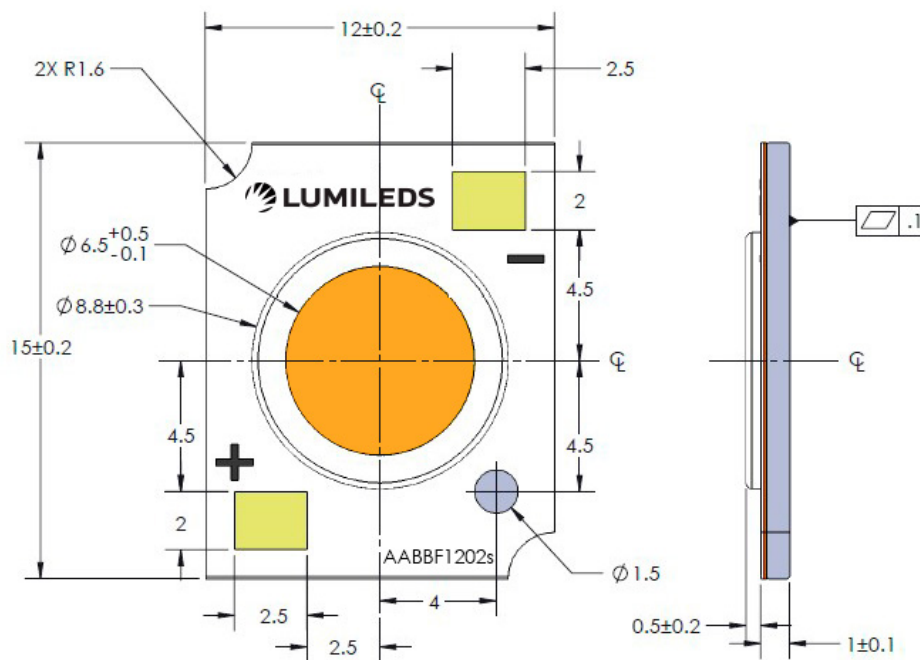
Figure 8a. Mechanical dimensions for L2C2-XXXX1202E0600.
